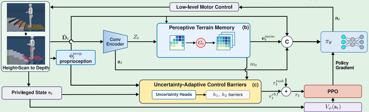
(a) DUALGuard overview
