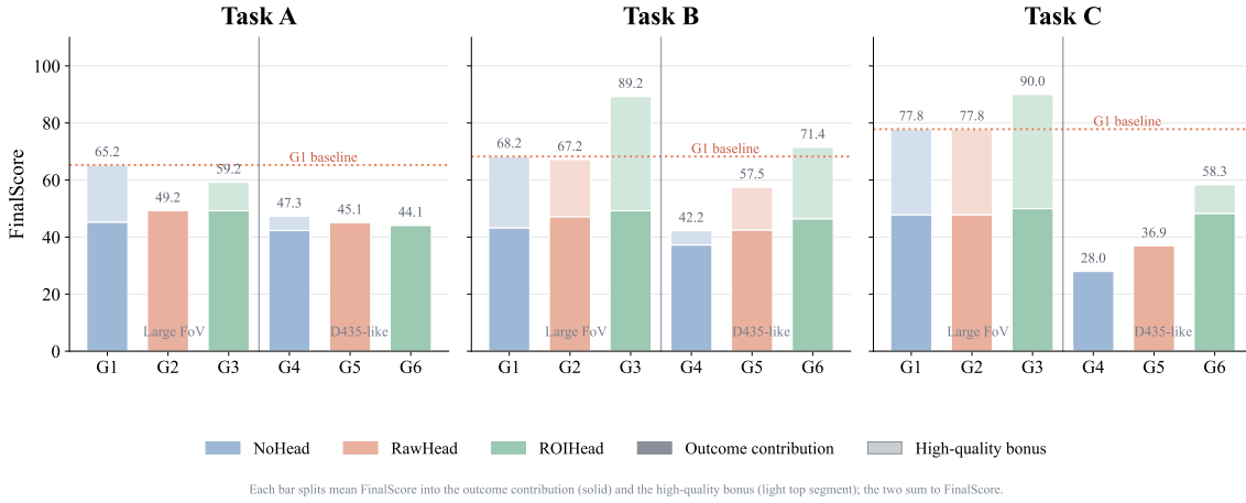
Figure 4 G1–G6 bar plots for the three tasks. Each bar shows FinalScore split into the outcome contribution (solid) and the high-quality bonus (light top segment), following the Score Split column in Table 4. Bars without a light segment complete rollouts without earning any high-quality bonus.
