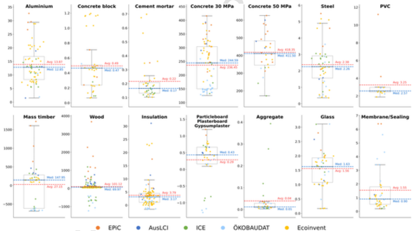
Fig. 1. GHG emissions factors for construction materials (kgCO 2 eq/m 3 for timber and concrete; kgCO 2 eq/kg for other materials).
