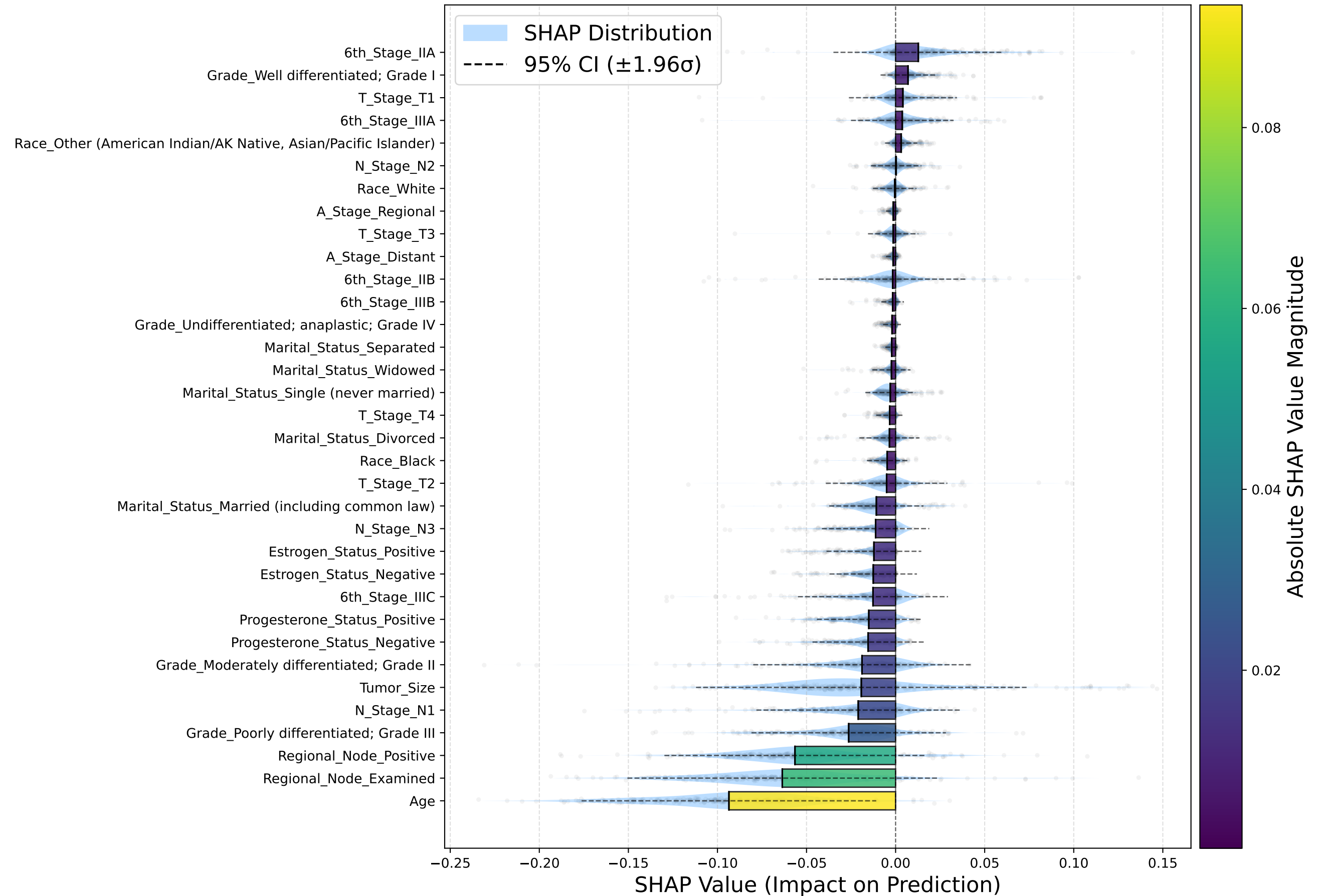
SHAP with Epistemic Uncertainty - Class: Dead
