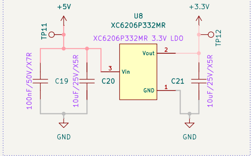
VDD 3.3V Voltage Regulator – XC6206P332MR
