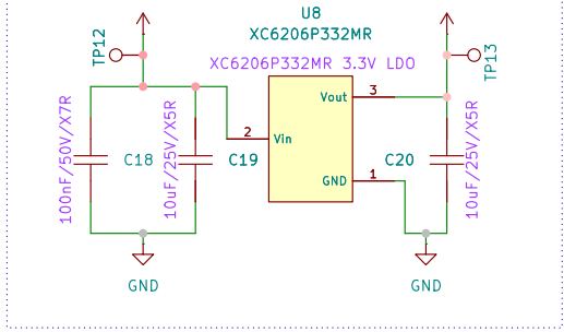
VDD 3.3V Voltage Regulator - XC6206P332MR
