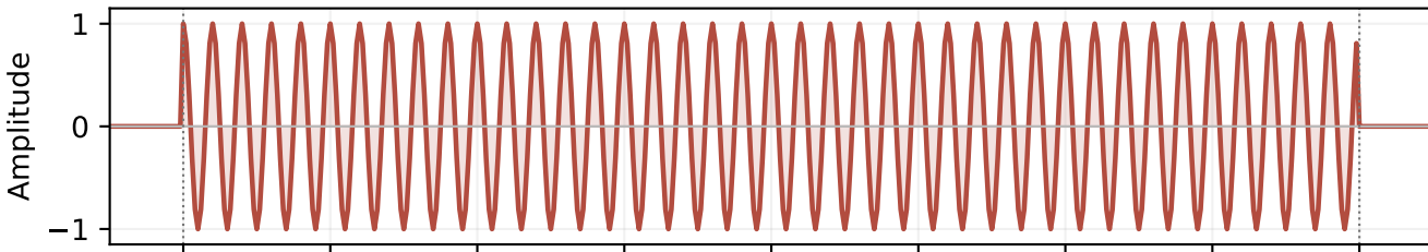
Without taper: abrupt finite-window edges
