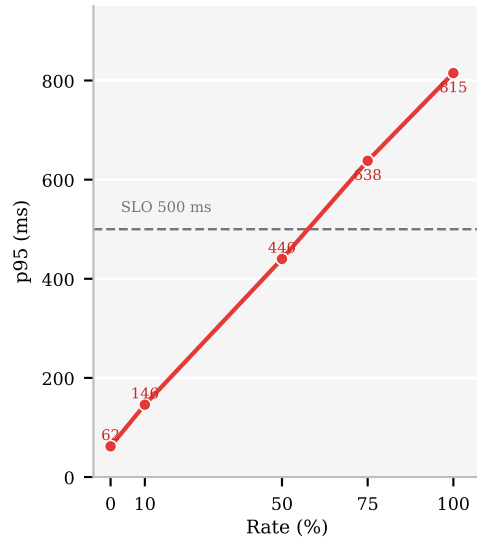
RQ3: Trace Overhead
