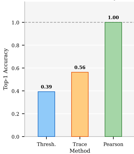
RQ2: RCA Accuracy
