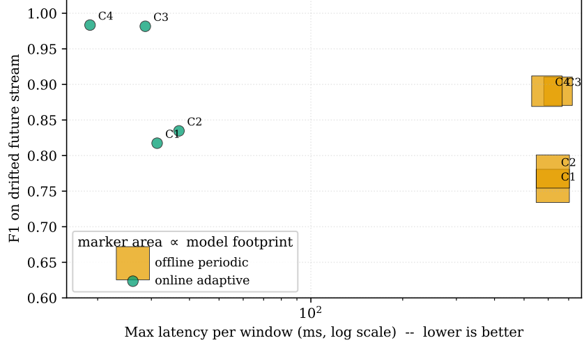
Fig. 6 RQ3 cost/quality trade-off (periodic vs. online). The online learner (green) sits top-left—higher F1 at an order-of-magnitude lower tail latency—with a tiny footprint (marker area \propto model size), while periodic retraining (orange) pays \sim 600 ms refit spikes and a multi-megabyte footprint for lower F1.
