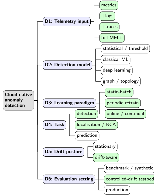
Fig. 1 A taxonomy of cloud-native anomaly detection along six dimensions—four of design (D1–D4) and two of evaluation (D5–D6). Shaded leaves mark the region the present study occupies: it holds the detection model fixed (D2) as a control while sweeping telemetry completeness (D1) and the learning paradigm (D3) together , evaluating detection and localisation under controlled drift (D5–D6). The bulk of prior work fixes D3 to static-batch and D5 to stationary.
