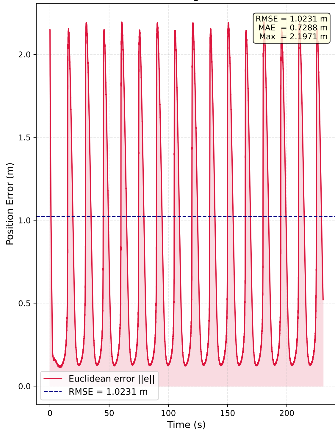
Euclidean Tracking Error vs Time
