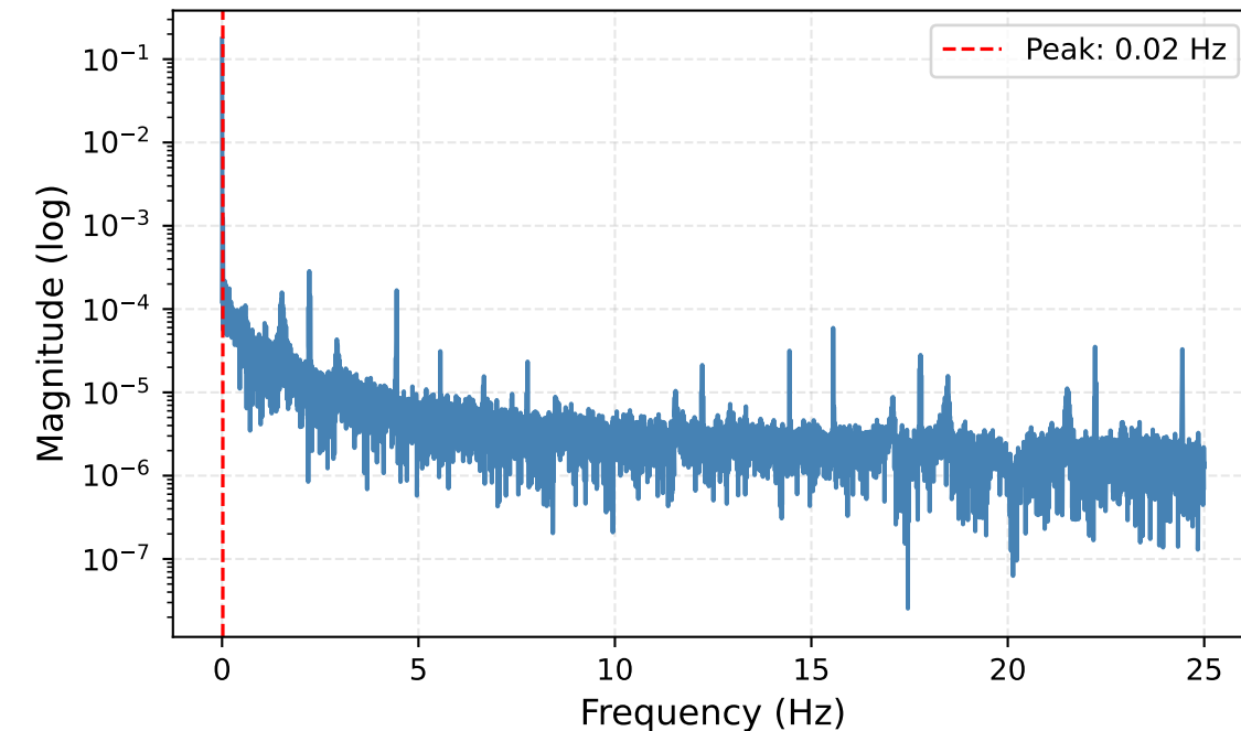
FFT — Linear Velocity
