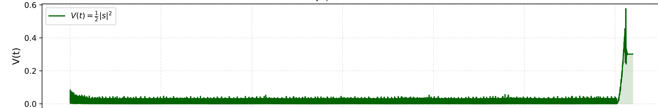
Lyapunov Function
