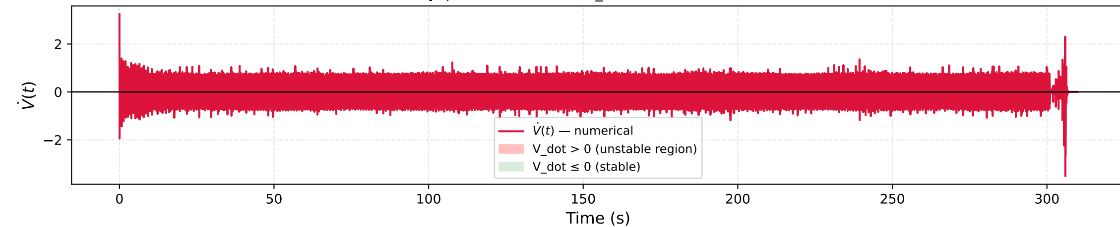
Lyapunov Derivative ( V_{\dot{}} \leq 0 : 52.9% of time)
