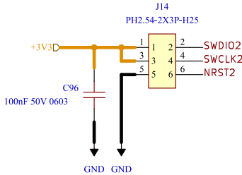
SWD Debug Connector
