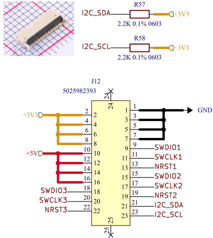
FFC Connector MCB & MB
