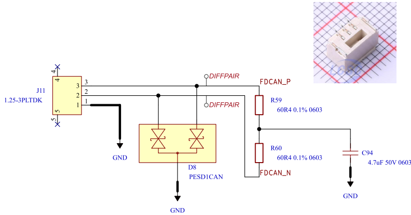
FD-CAN Connector and Termination
