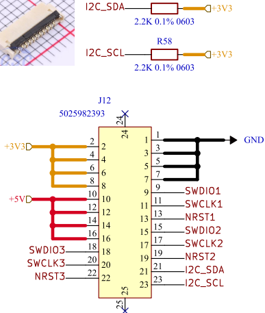
FFC Connector MCB & MB
