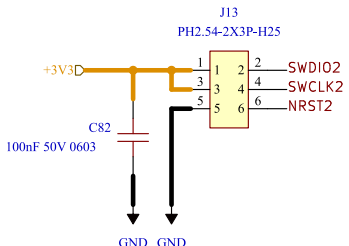
SWD Debug Connector
