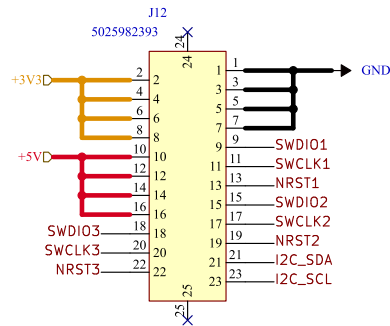
FFC Connector MCB & MB
