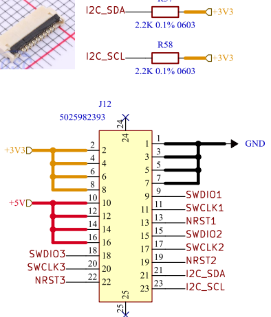
FFC Connector MCB & MB
