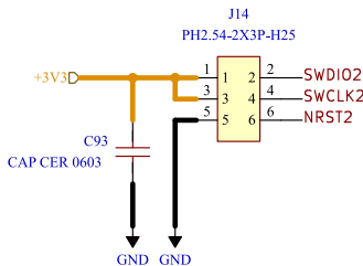
SWD Debug Connector
