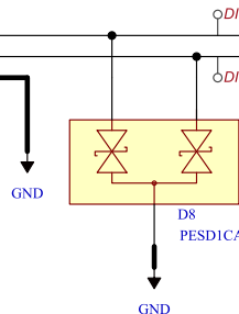
FD-CAN Connector and Termination
