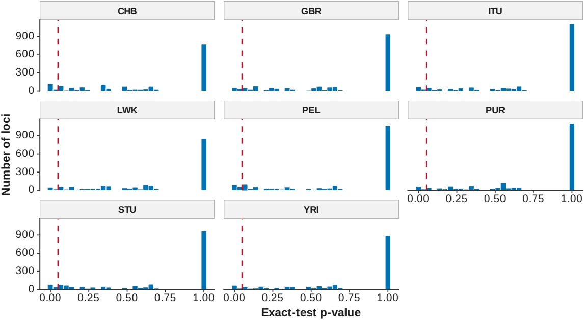
Figure 60: HWE p-values
