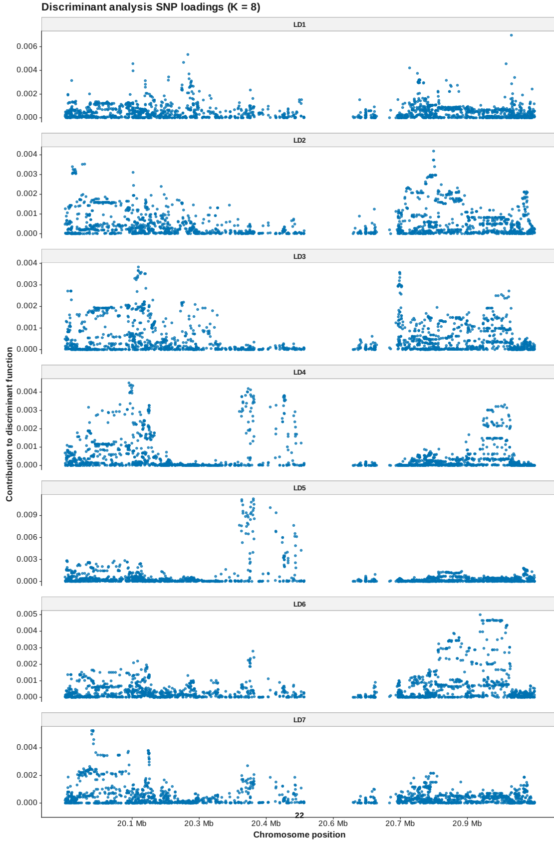
Figure 100: DAPC loadings manhattan K 8
