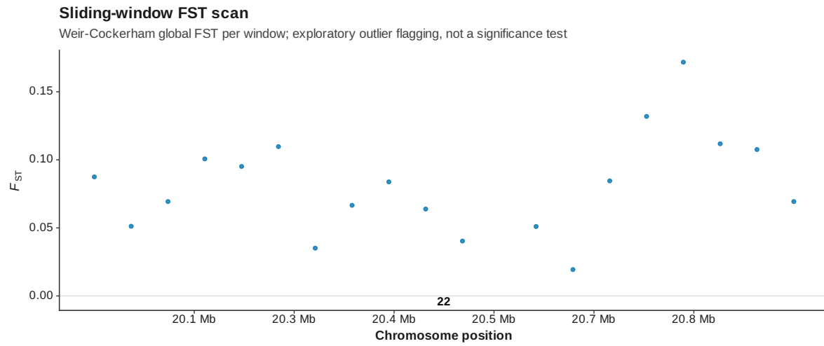
Figure 120: Genome scan FST manhattan
