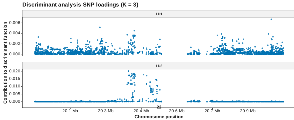
Figure 95: DAPC loadings manhattan K 3
