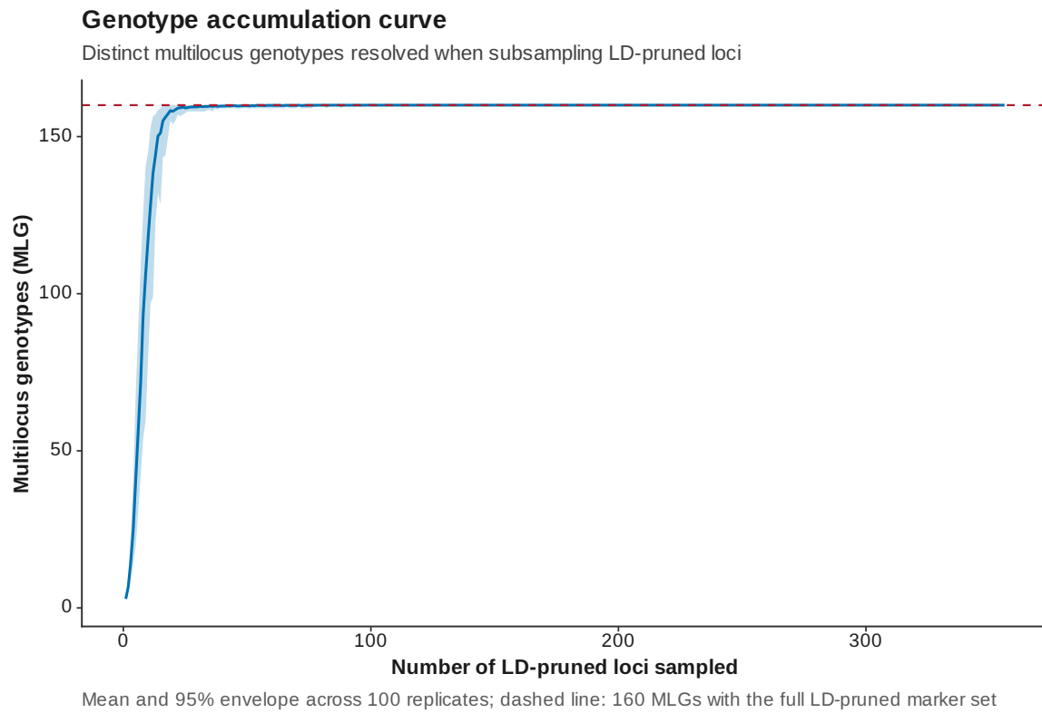
Figure 151: Genotype accumulation curve
