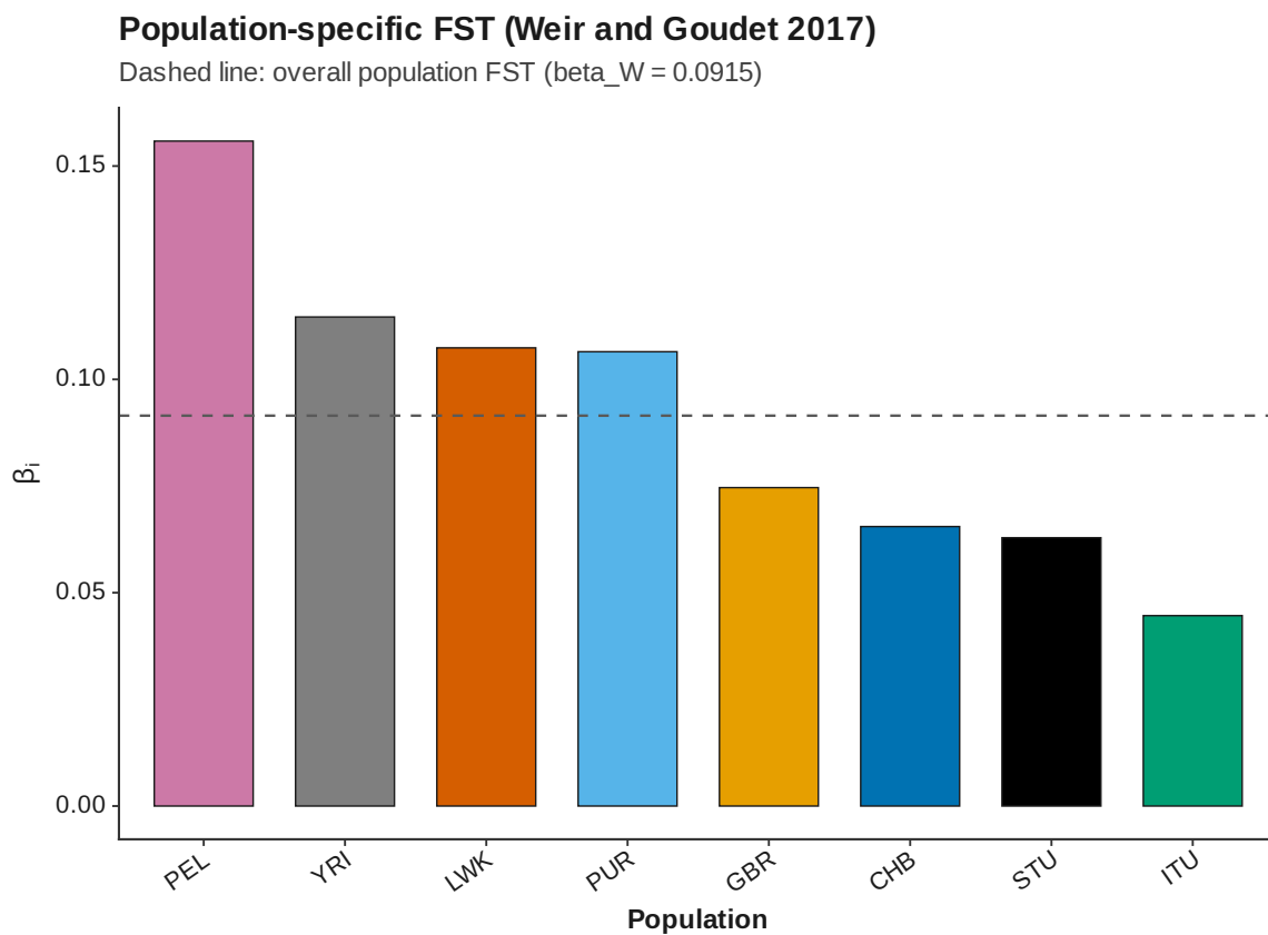
Figure 147: Population specific fst
