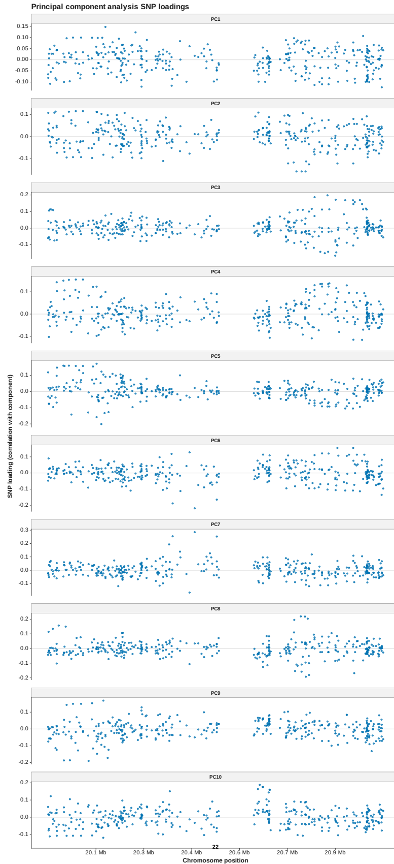
Figure 130: PCA loadings manhattan
