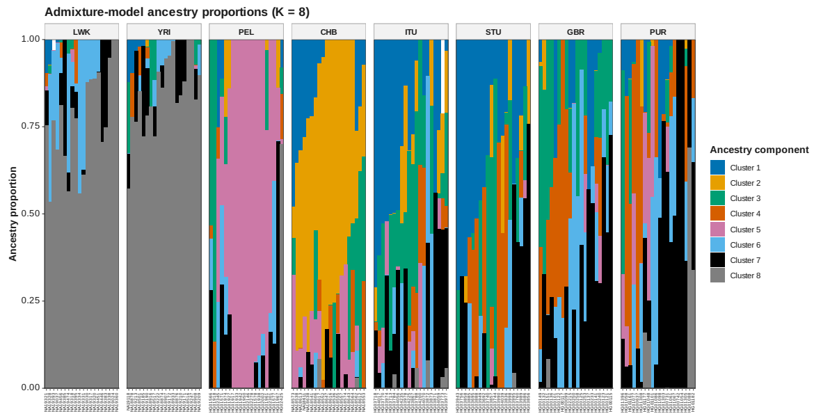
Figure 60: ADMIXTURE Q K 8
