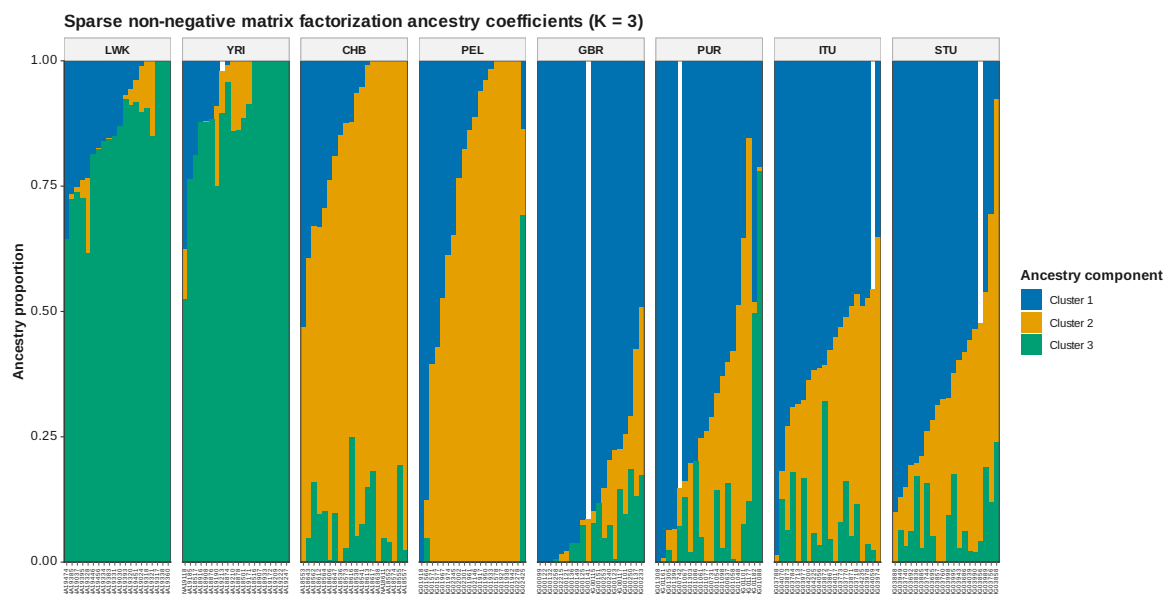
Figure 105: SNMF Q K 3
