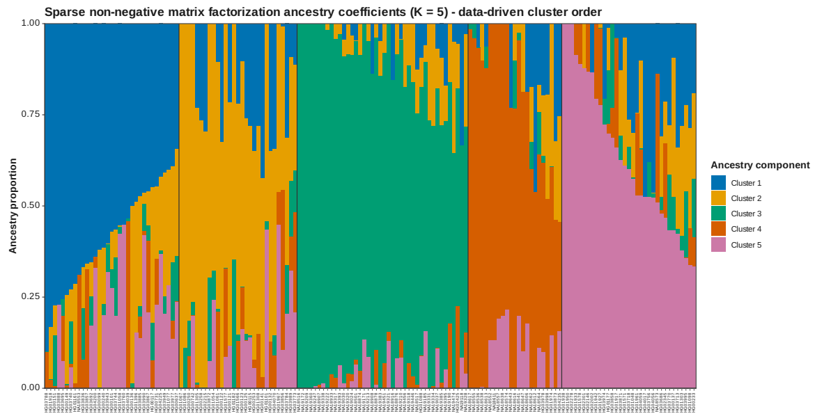
Figure 99: SNMF Q data driven K 5
