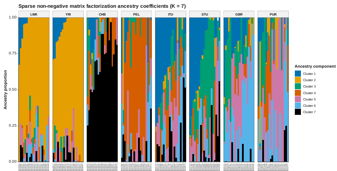
Figure 109: SNMF Q K 7
