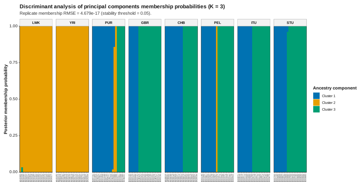
Figure 72: DAPC membership K 3
