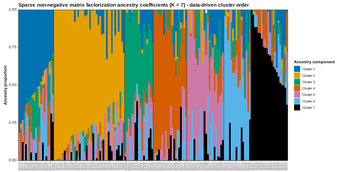
Figure 101: SNMF Q data driven K 7
