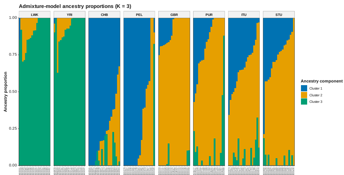
Figure 55: ADMIXTURE Q K 3
