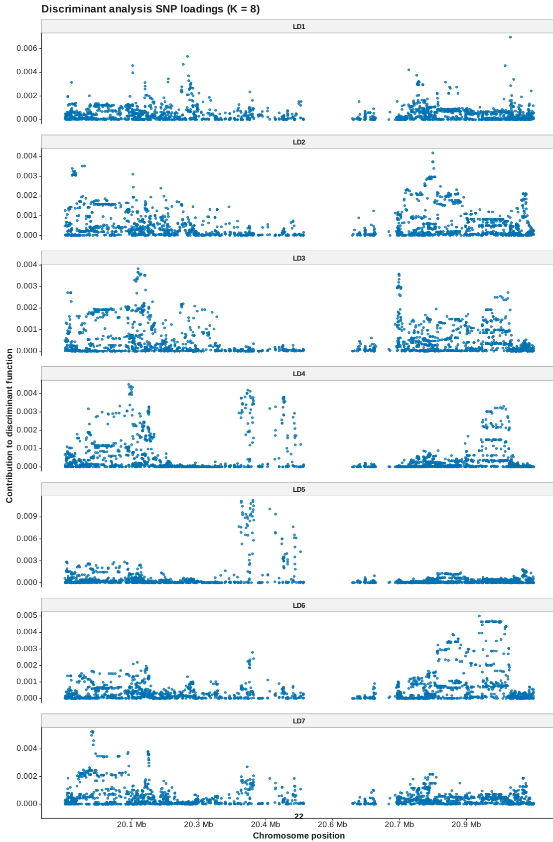
Figure 118: DAPC loadings manhattan K 8
