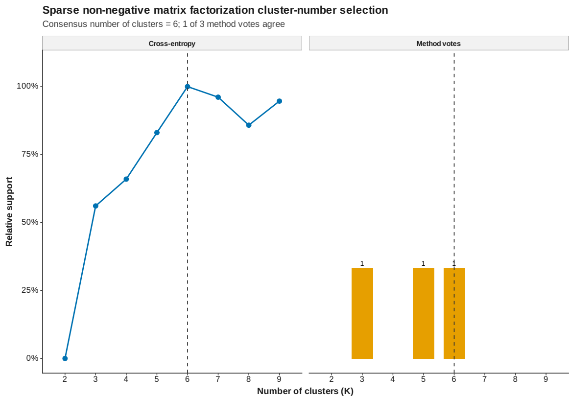
Figure 44: SNMF cluster number selection
