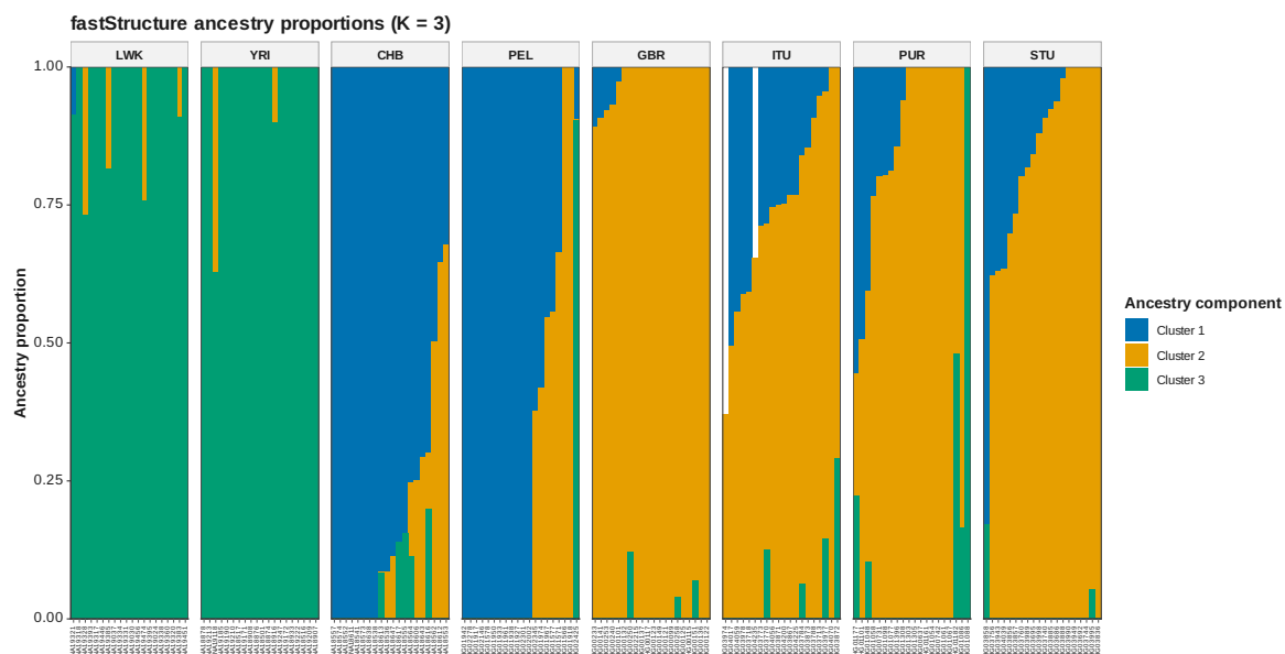
Figure 89: FastStructure Q K 3
