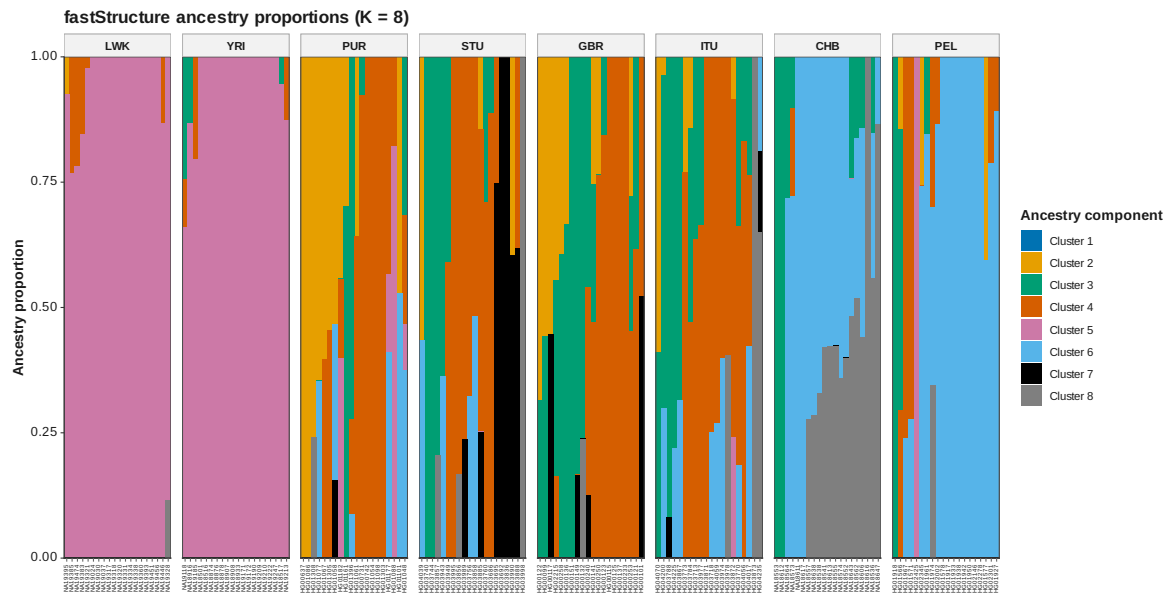
Figure 94: FastStructure Q K 8
