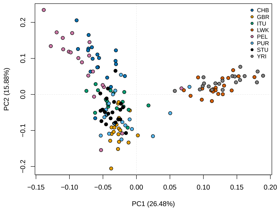
Figure 155: PCA PC 1 PC 2
