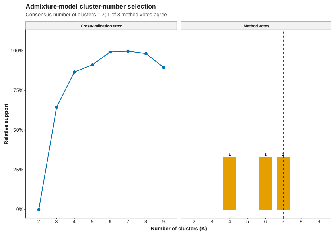
Figure 43: ADMIXTURE cluster number selection
