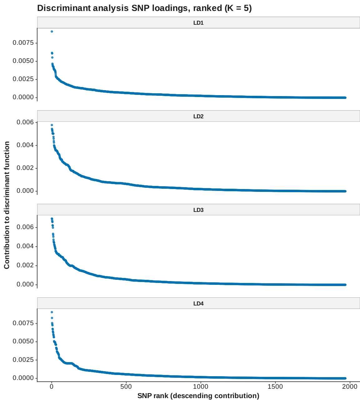
Figure 124: DAPC loadings ranked K 5
