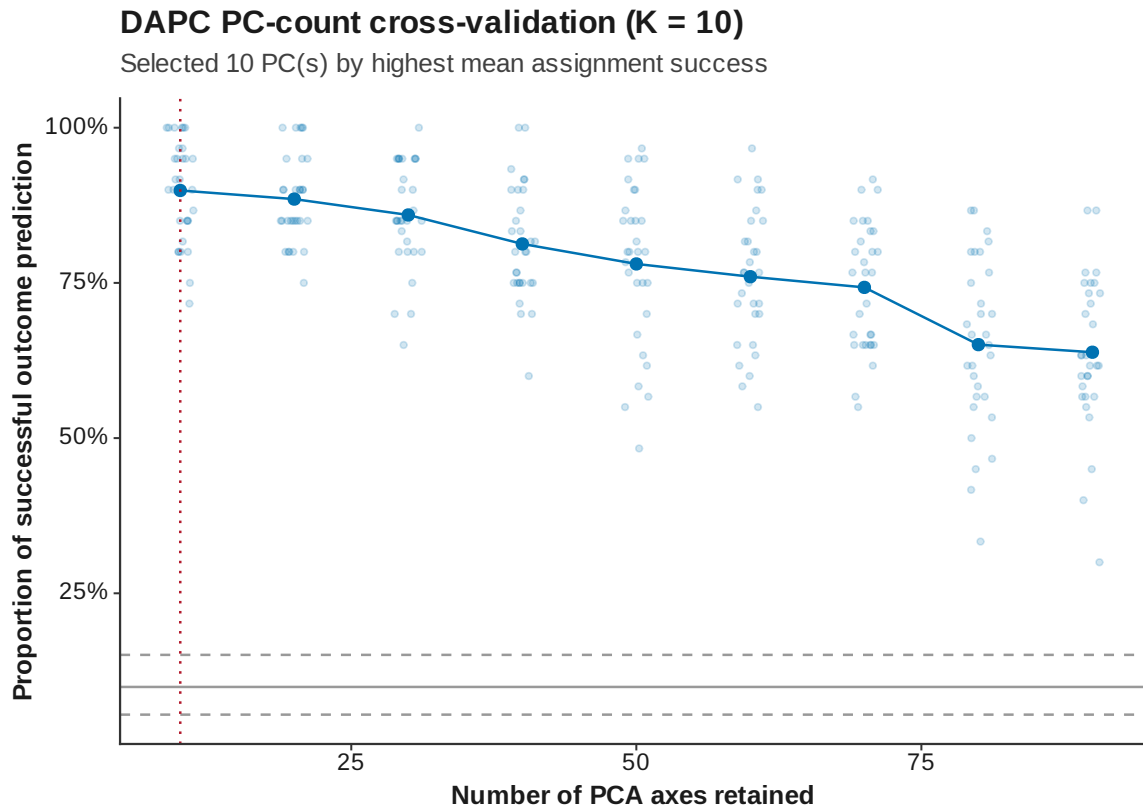
Figure 32: DAPC xval K 10
