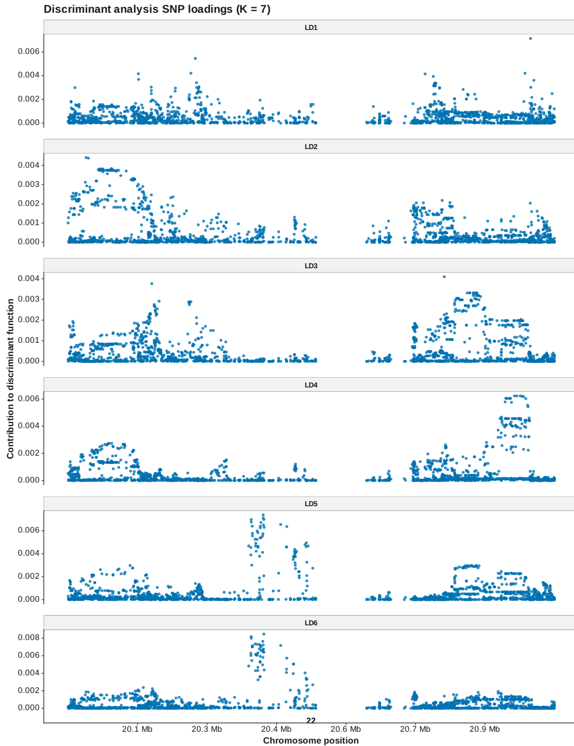
Figure 117: DAPC loadings manhattan K 7
