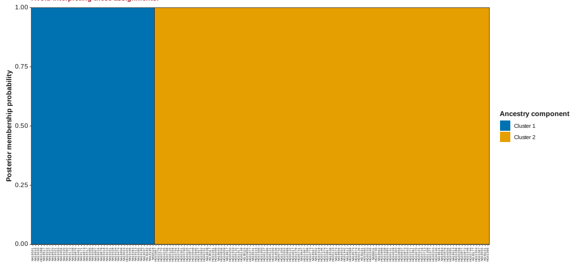
Figure 62: DAPC membership data driven K 2
