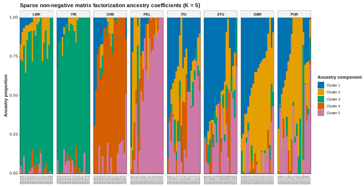
Figure 107: SNMF Q K 5
