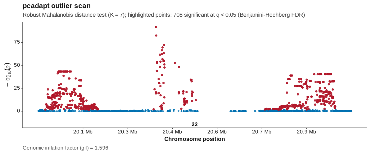
Figure 153: Pcadapt manhattan
