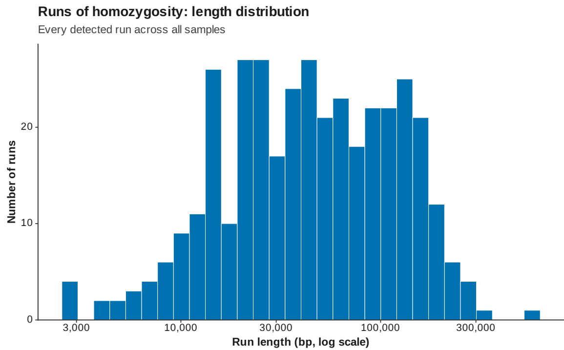
Figure 135: ROH length distribution
