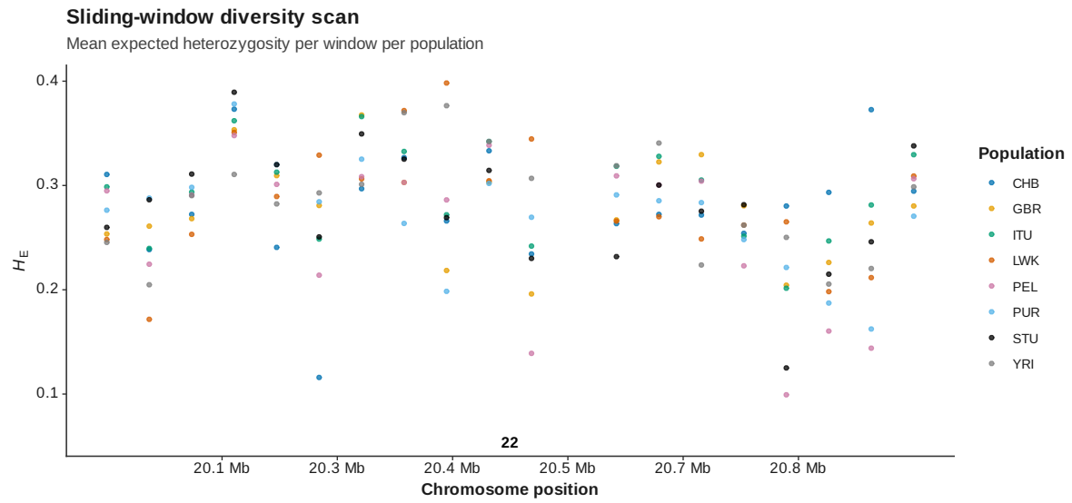
Figure 139: Genome scan diversity manhattan
