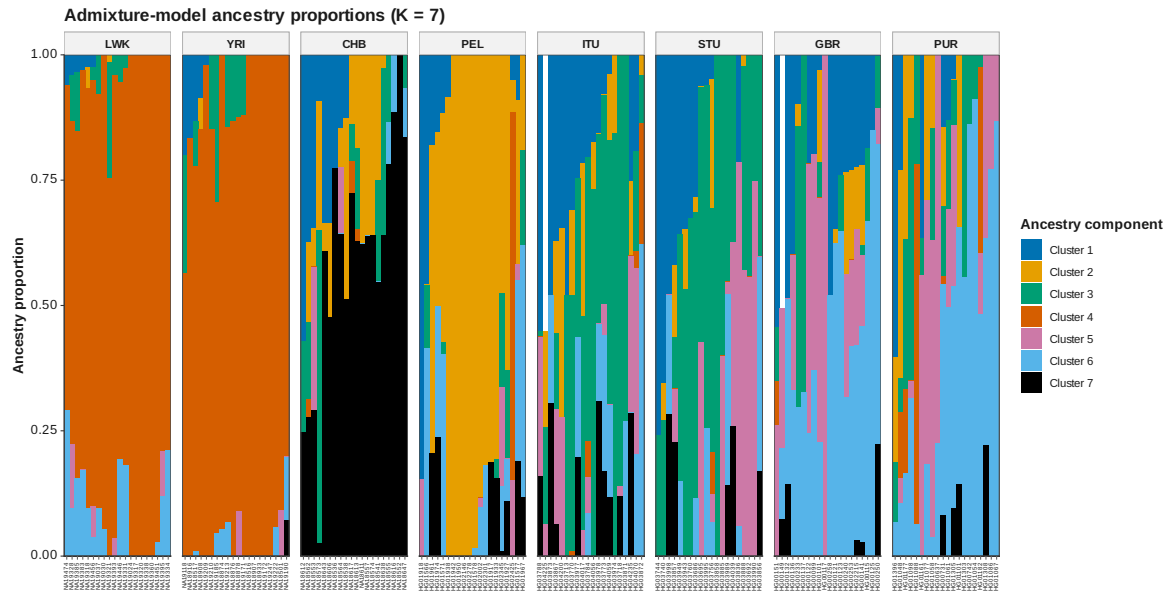
Figure 59: ADMIXTURE Q K 7
