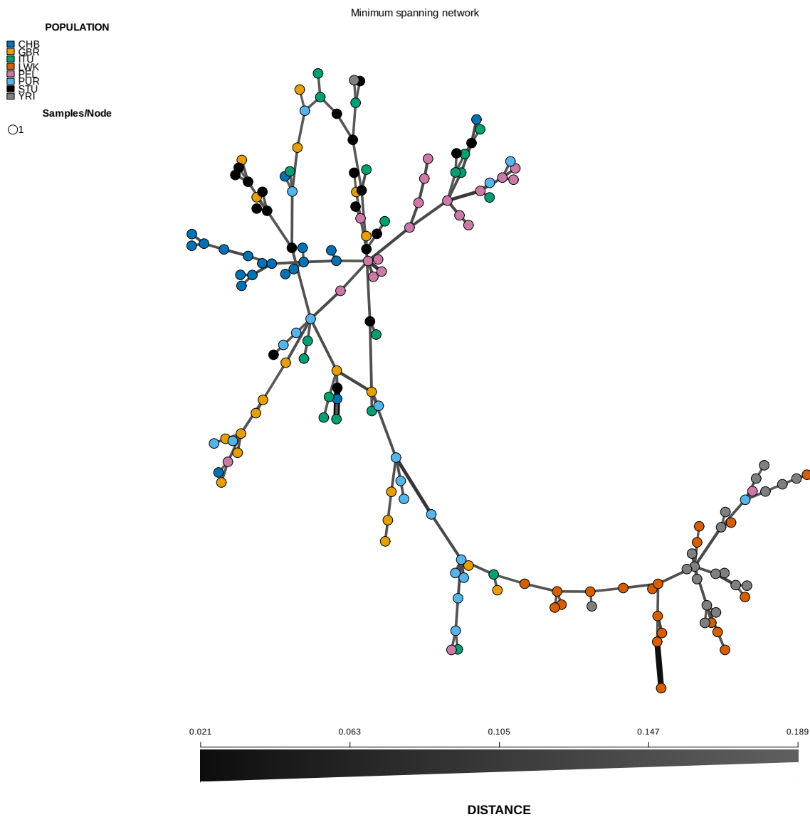
Figure 152: MSN network
