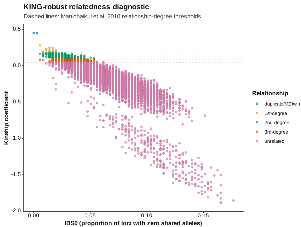
Figure 134: Kinship IBS 0 vs kinship
