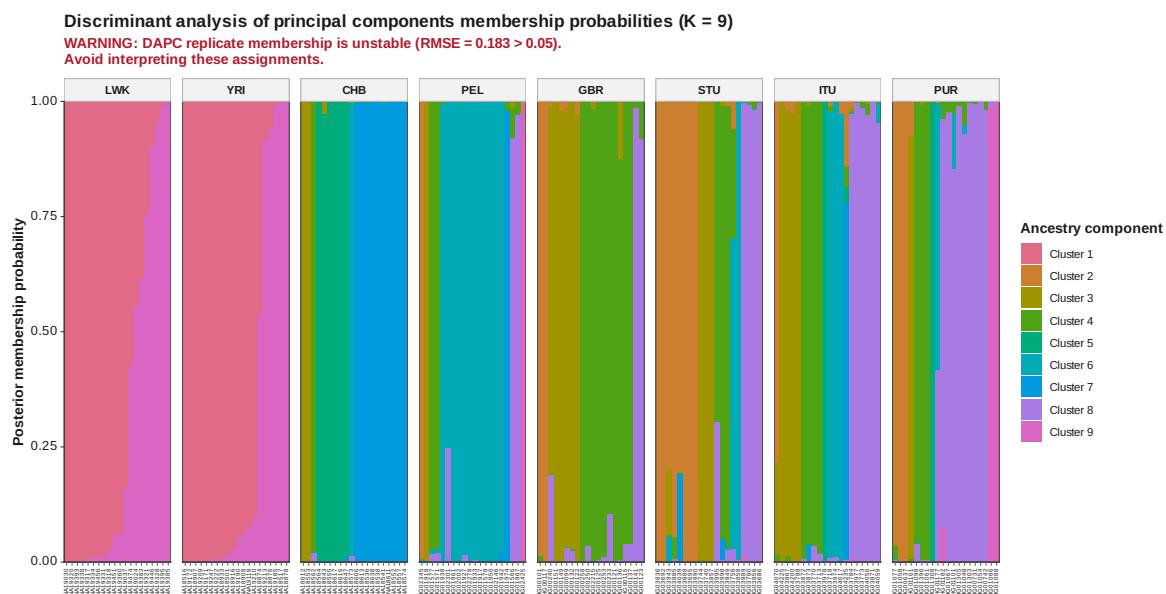
Figure 78: DAPC membership K 9
