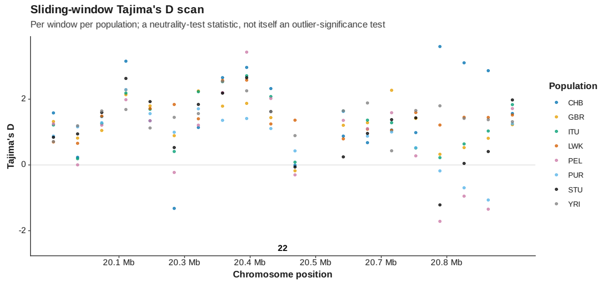
Figure 140: Genome scan tajima d manhattan
