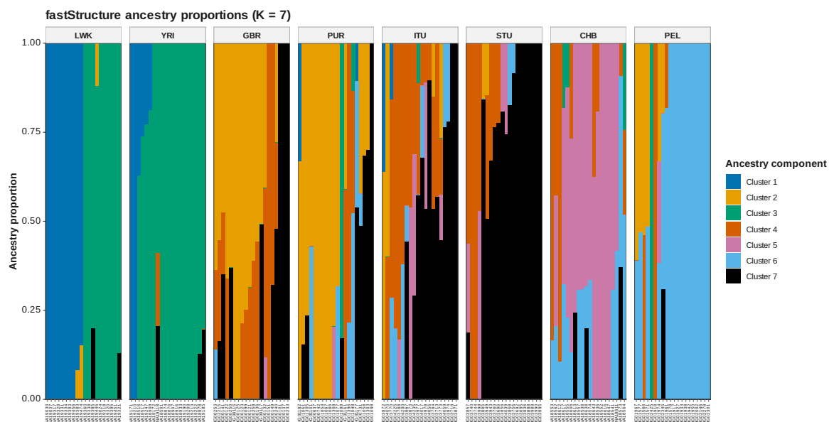
Figure 93: FastStructure Q K 7
