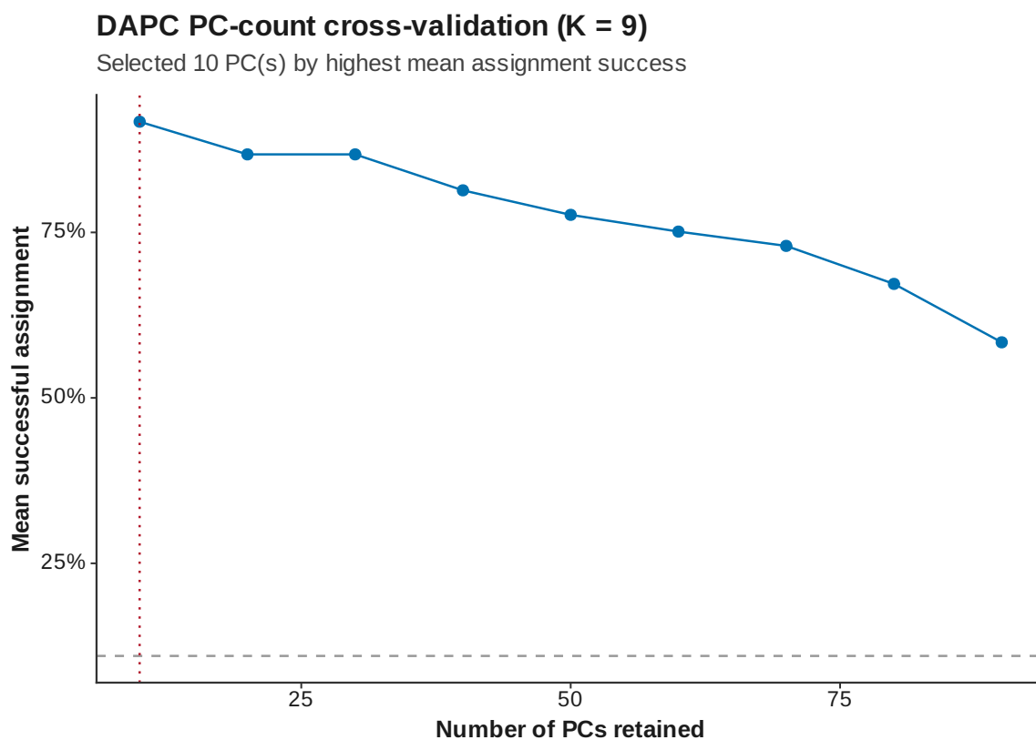
Figure 31: DAPC xval K 9
