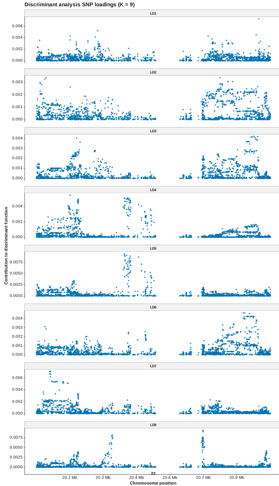
Figure 110: DAPC loadings manhattan K 9
