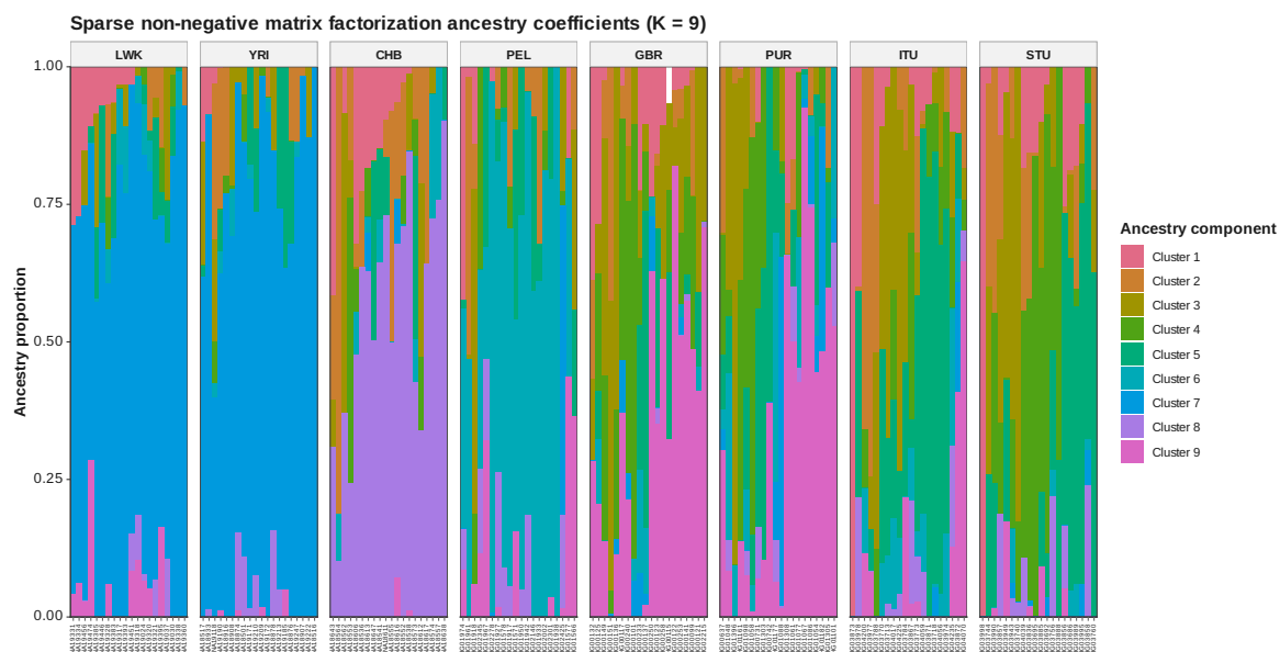
Figure 102: SNMF Q K 9
