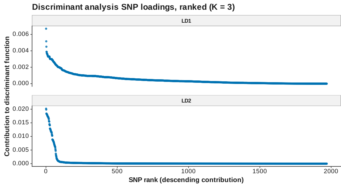
Figure 113: DAPC loadings ranked K 3
