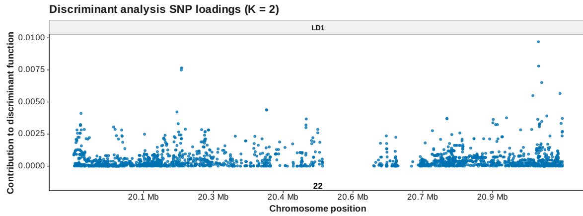
Figure 103: DAPC loadings manhattan K 2
