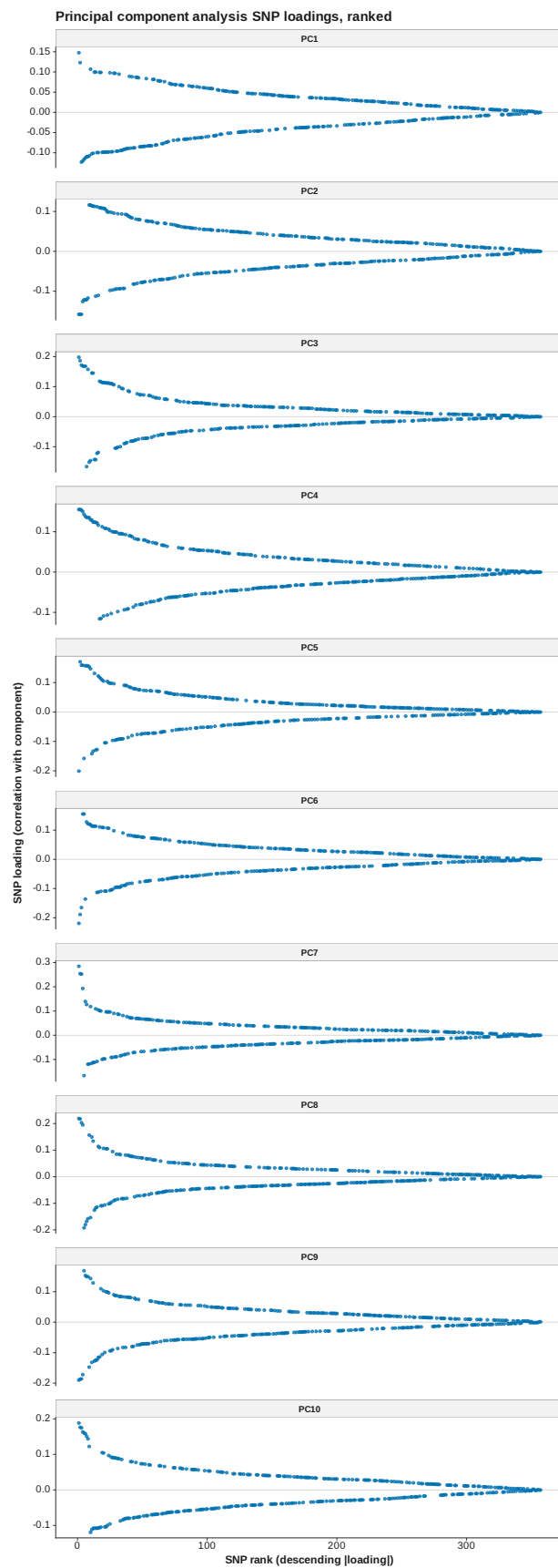
Figure 122: PCA loadings ranked
