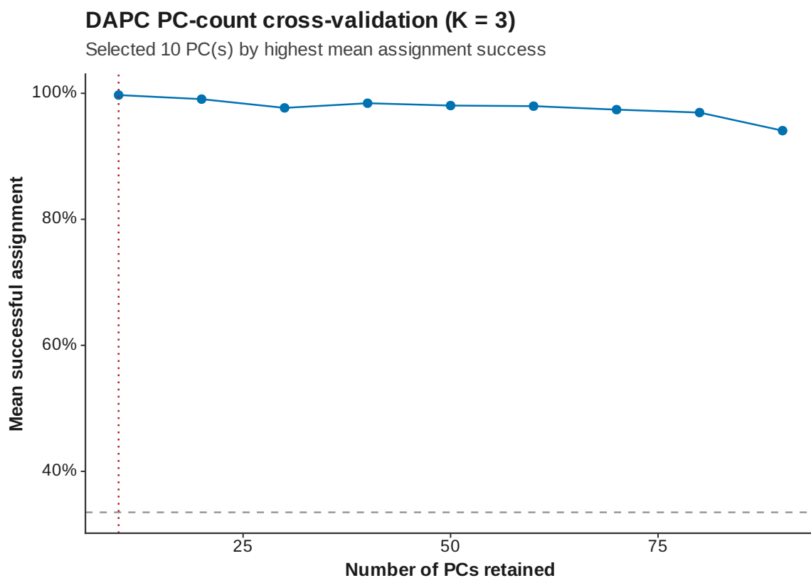
Figure 25: DAPC xval K 3
