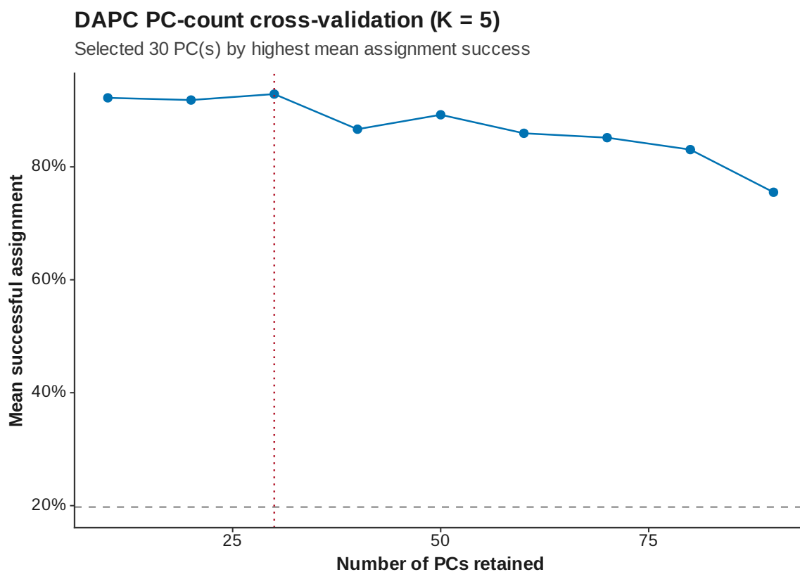
Figure 27: DAPC xval K 5
