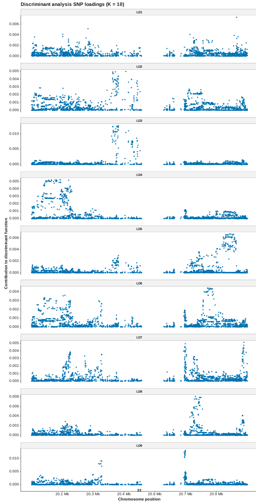
Figure 111: DAPC loadings manhattan K 10
