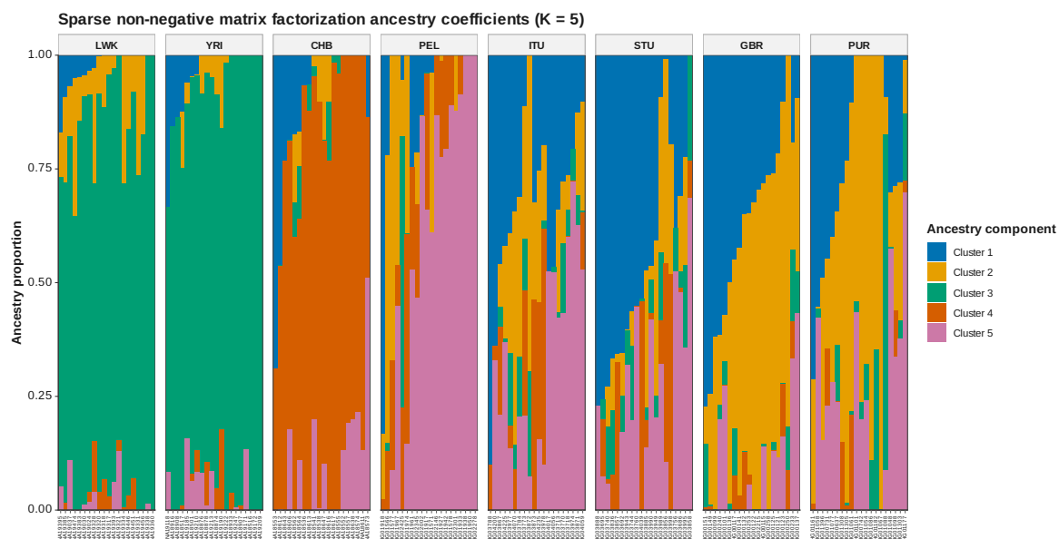
Figure 98: SNMF Q K 5
