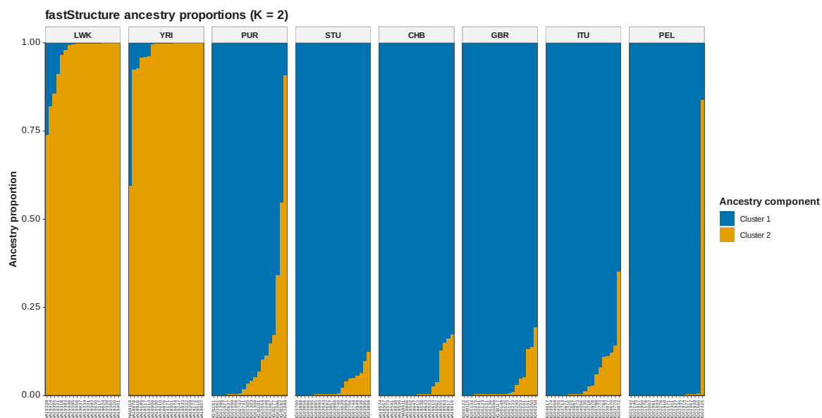
Figure 79: FastStructure Q K 2
