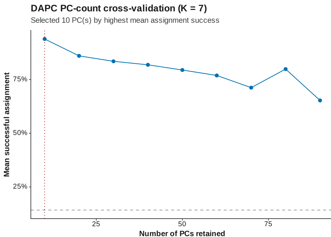
Figure 29: DAPC xval K 7
