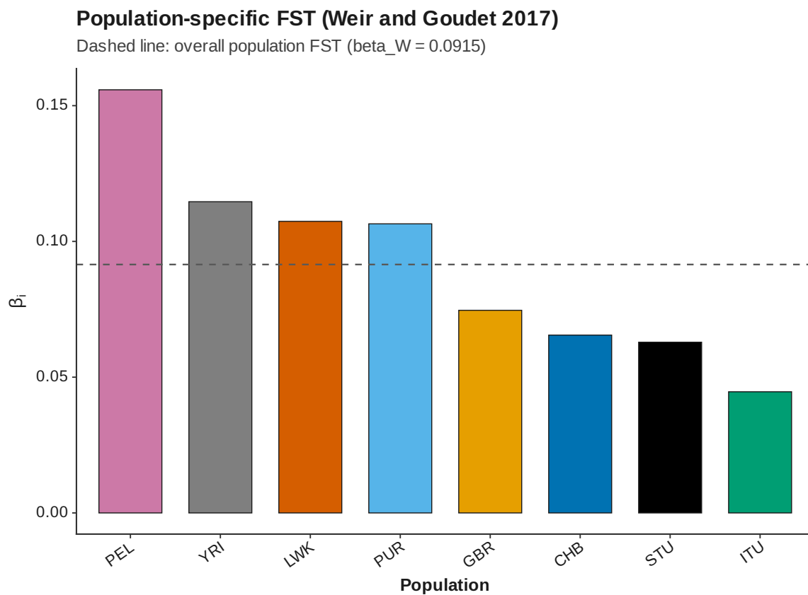
Figure 138: Population specific fst
