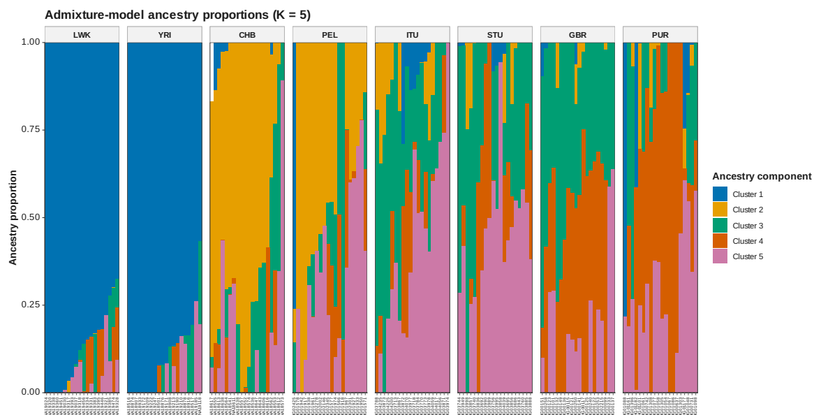
Figure 48: ADMIXTURE Q K 5
