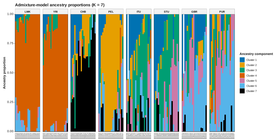
Figure 50: ADMIXTURE Q K 7
