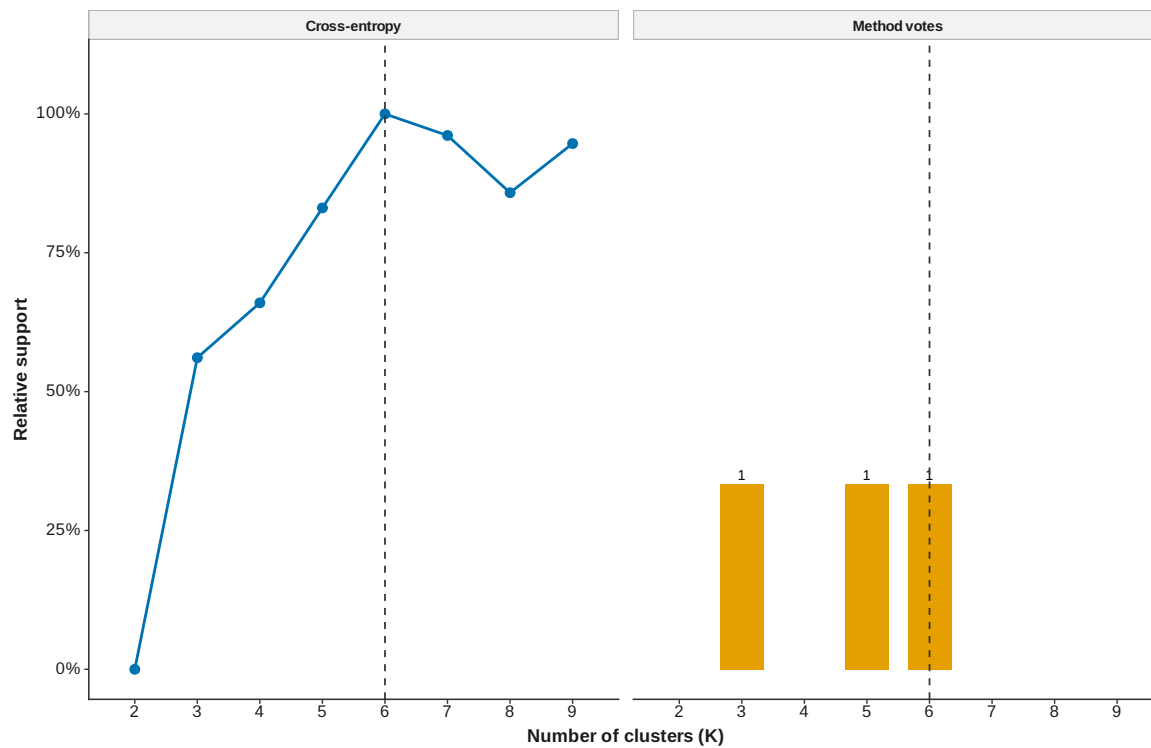
Figure 35: SNMF cluster number selection
