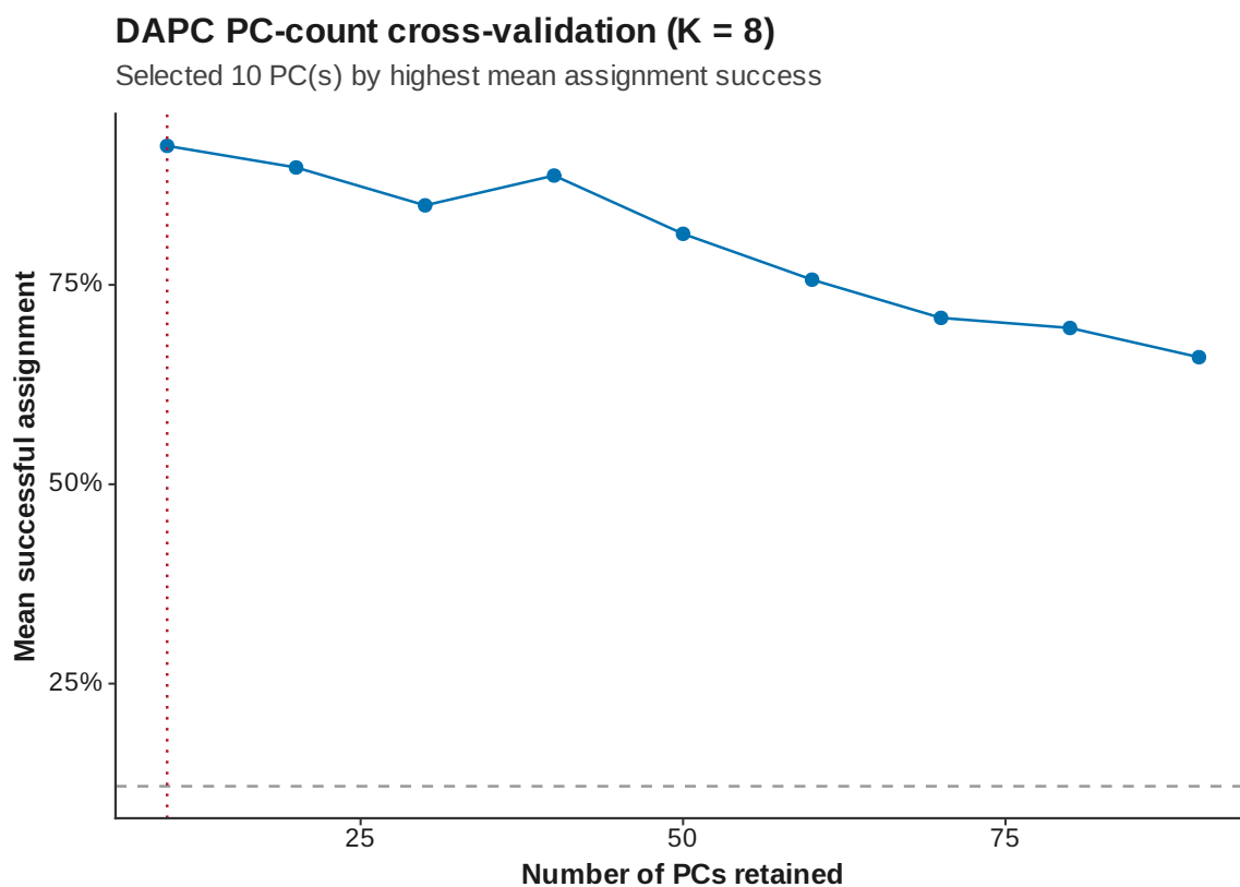
Figure 30: DAPC xval K 8
