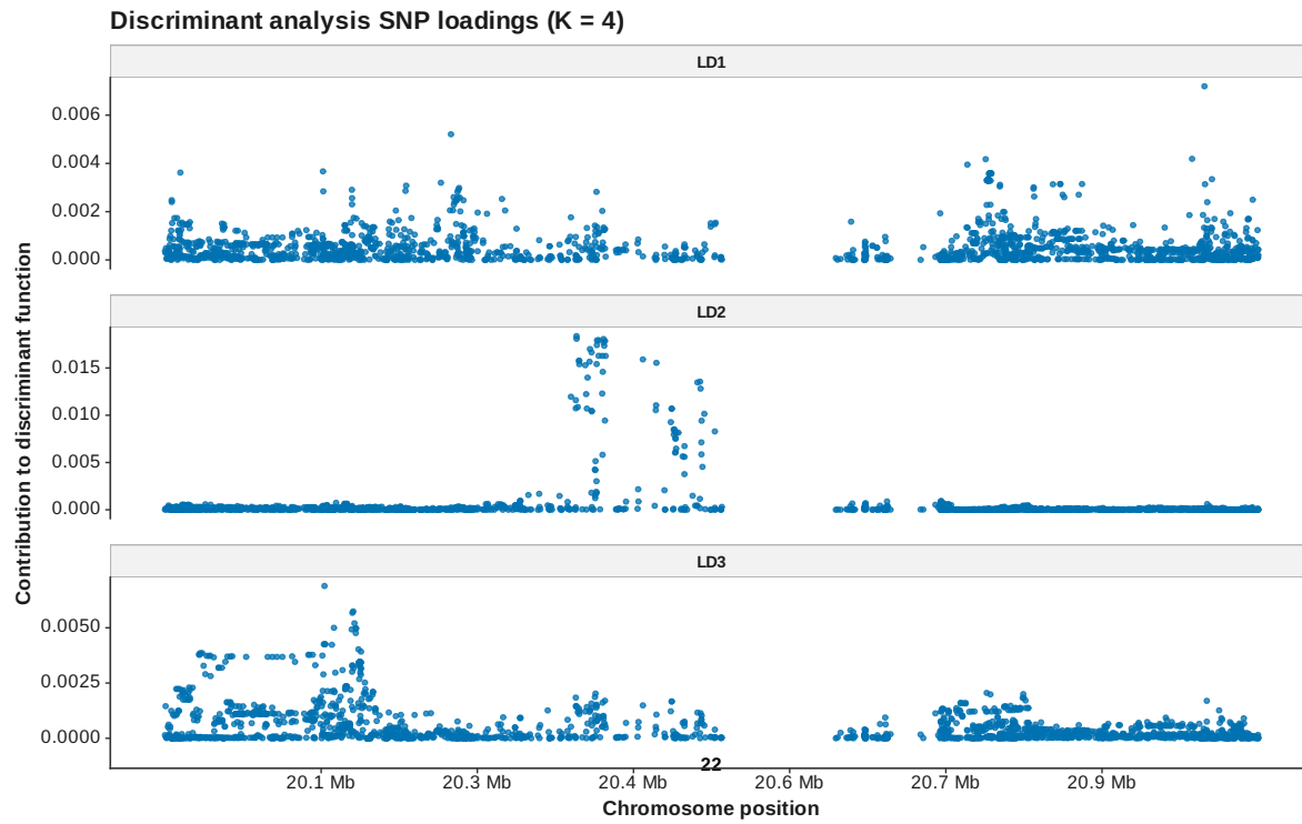
Figure 105: DAPC loadings manhattan K 4
