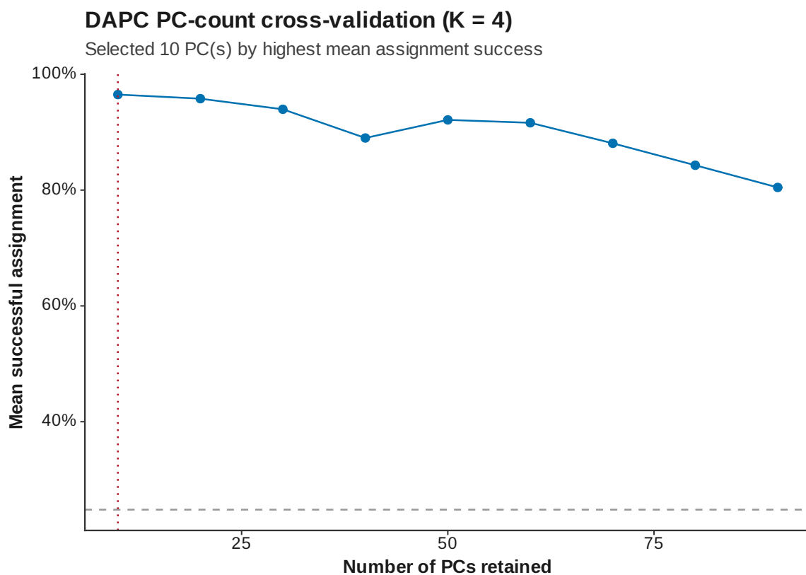
Figure 26: DAPC xval K 4
