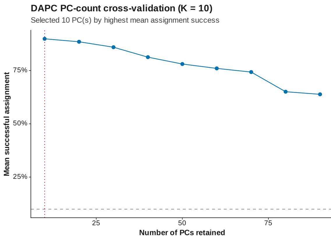
Figure 32: DAPC xval K 10
