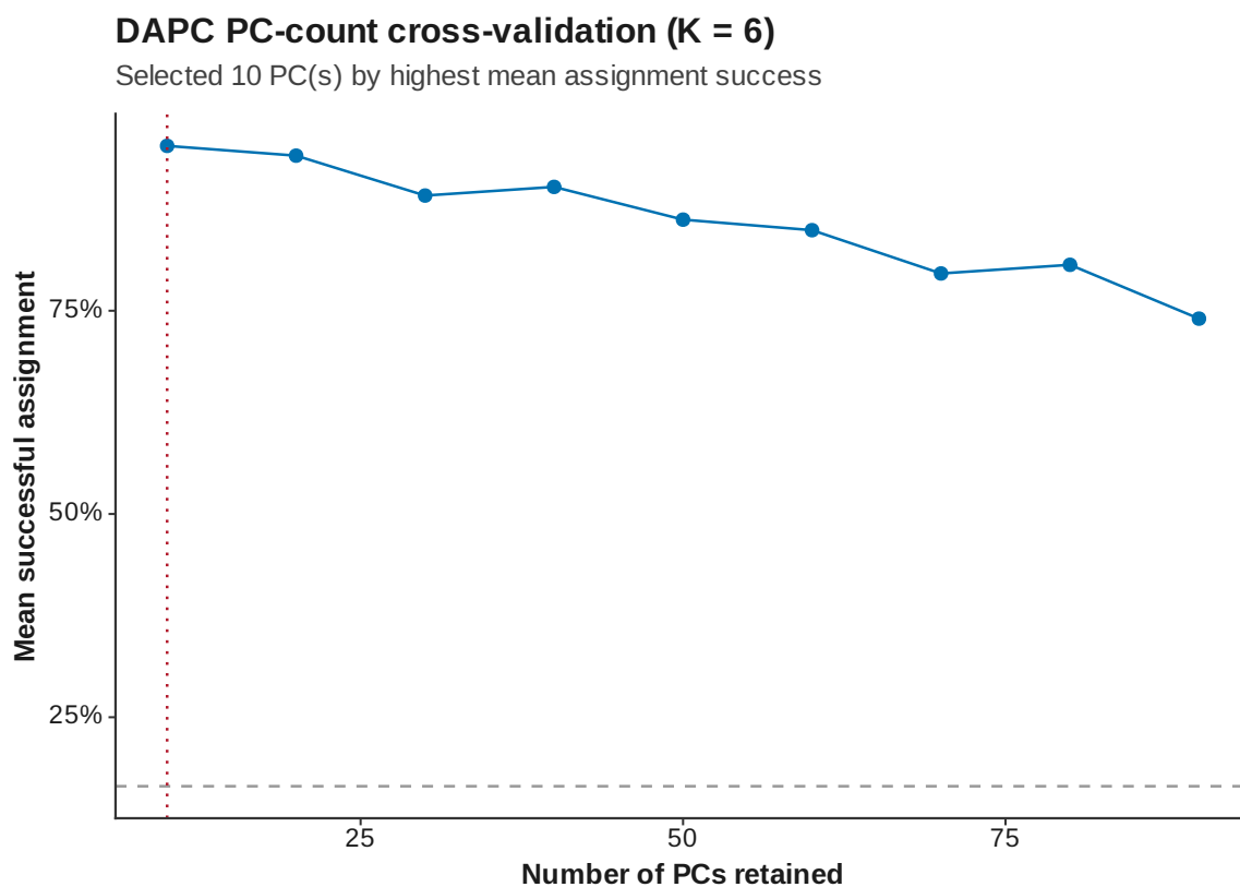
Figure 28: DAPC xval K 6
