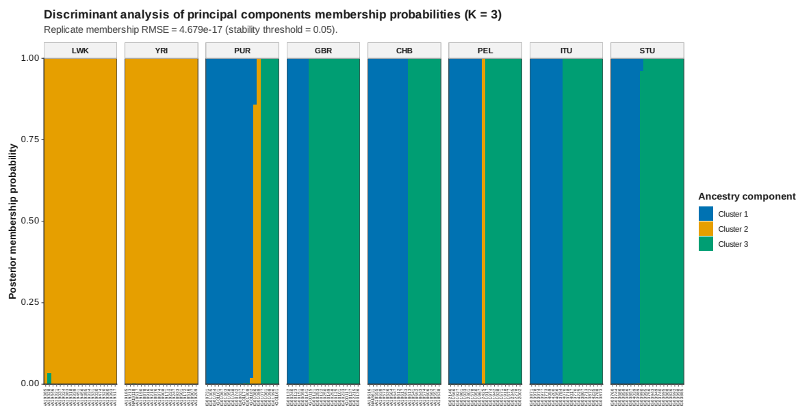
Figure 63: DAPC membership K 3
