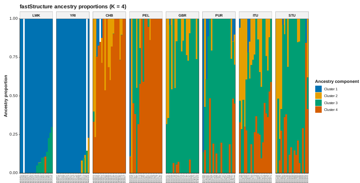
Figure 81: FastStructure Q K 4
