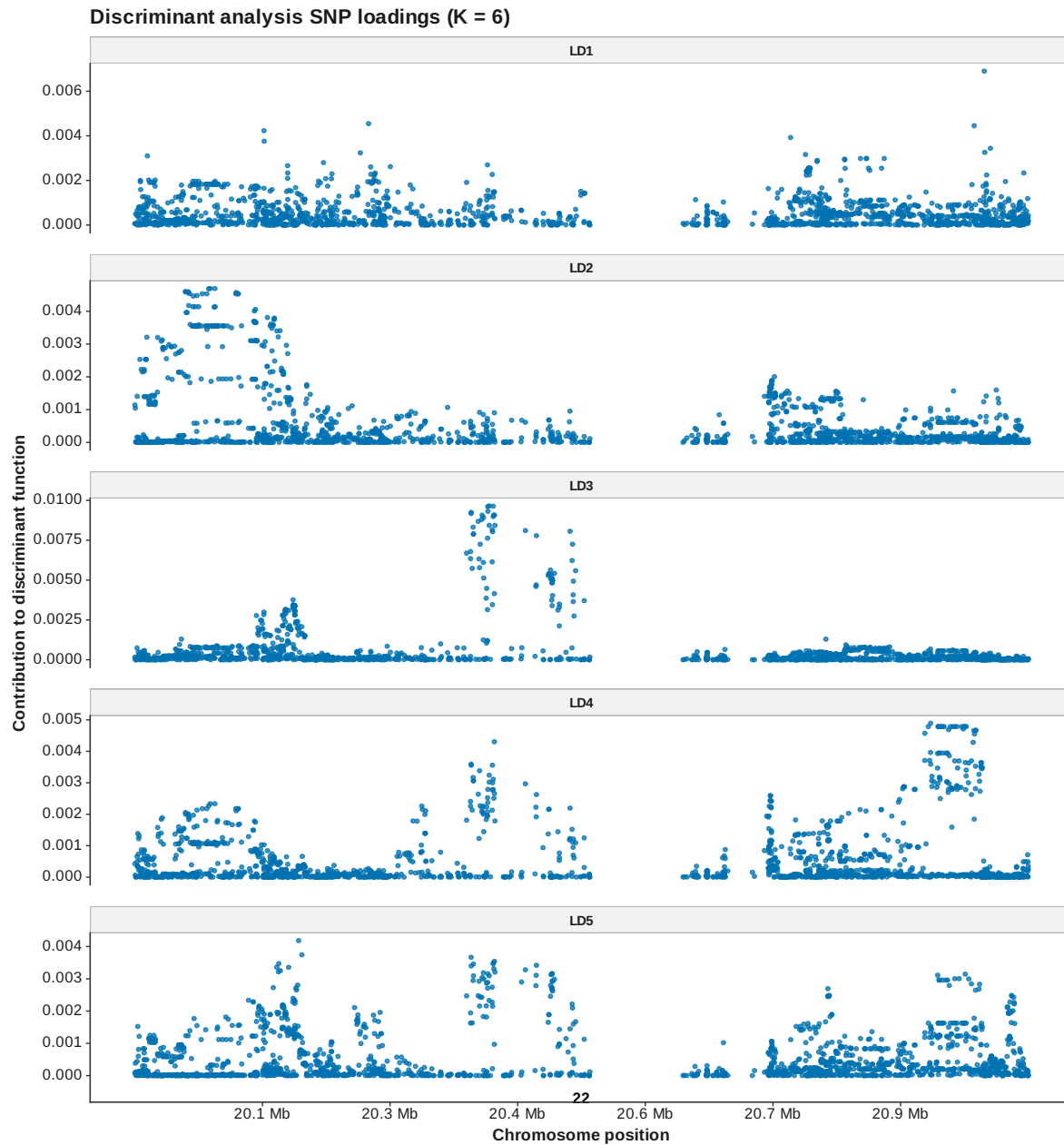
Figure 107: DAPC loadings manhattan K 6
