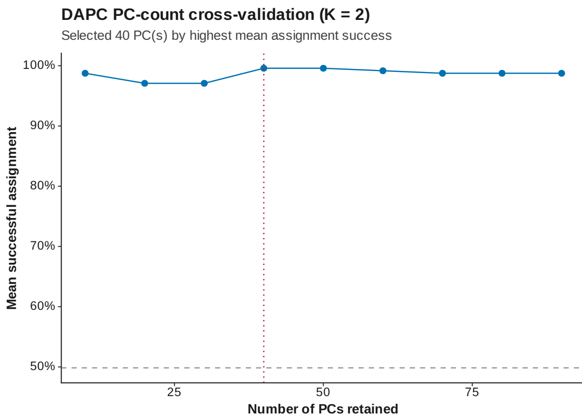
Figure 24: DAPC xval K 2
