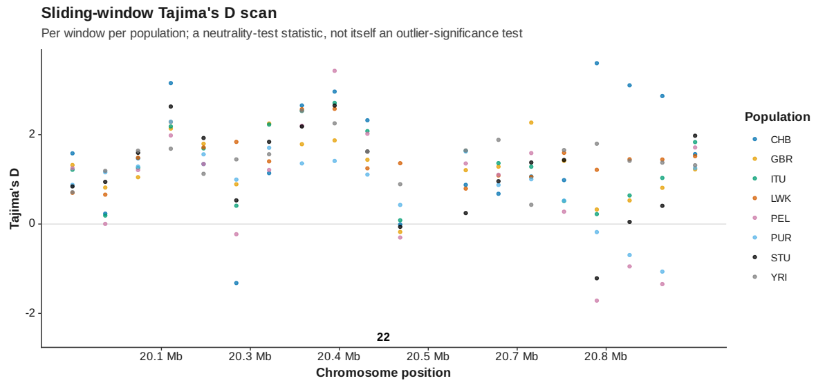
Figure 131: Genome scan tajima d manhattan
