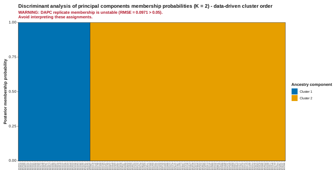
Figure 53: DAPC membership data driven K 2
