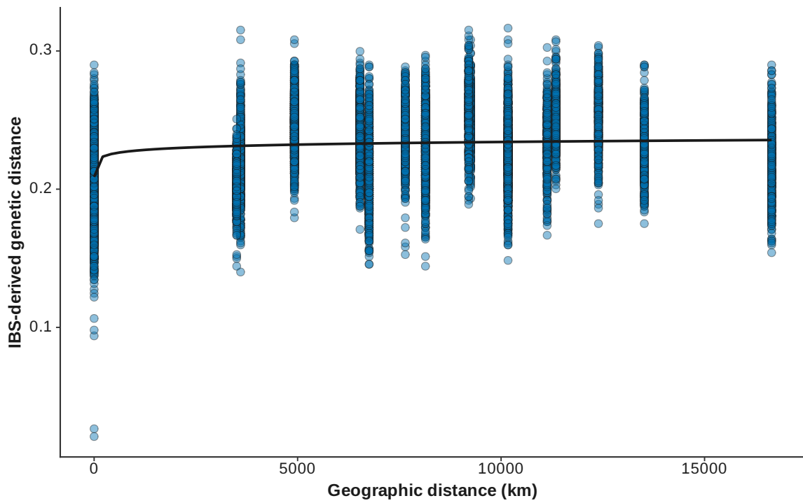
Figure 23: Isolation by distance
