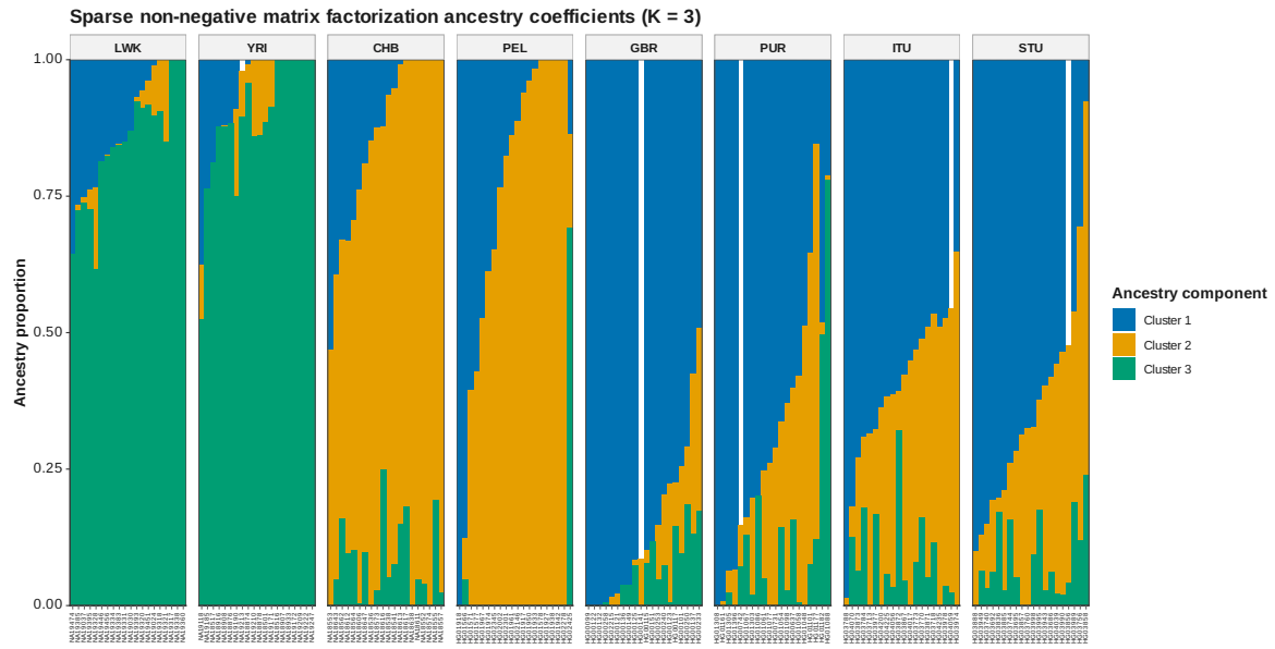
Figure 96: SNMF Q K 3
