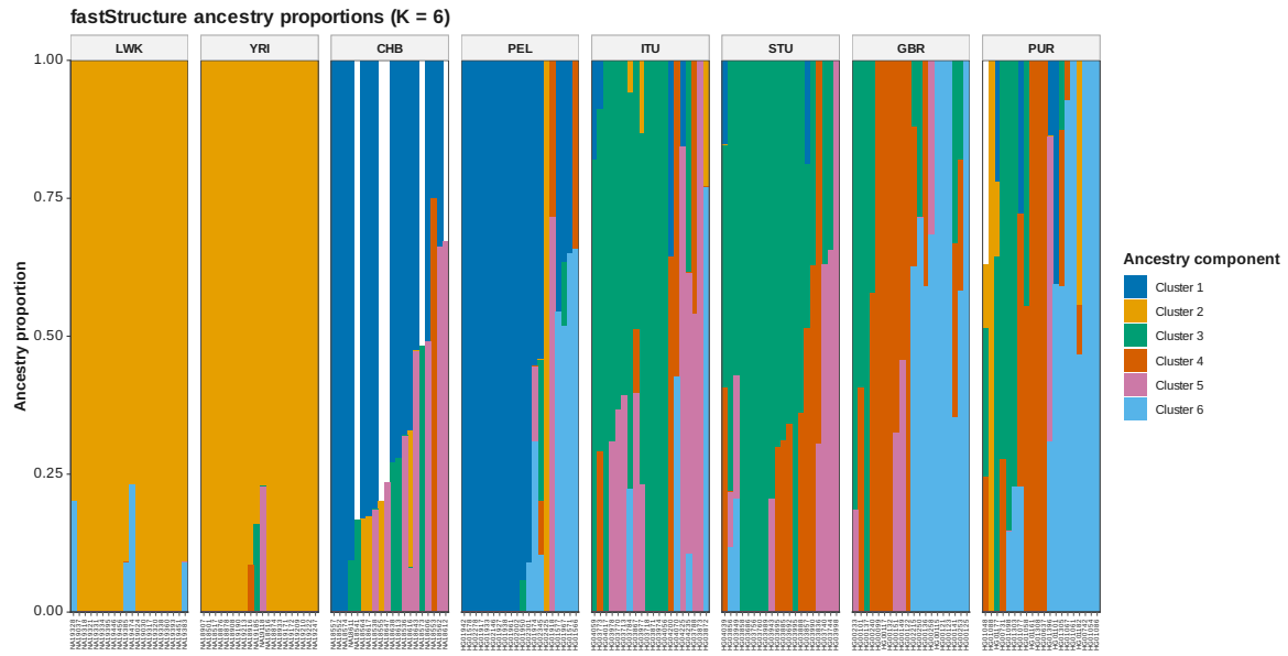
Figure 83: FastStructure Q K 6
