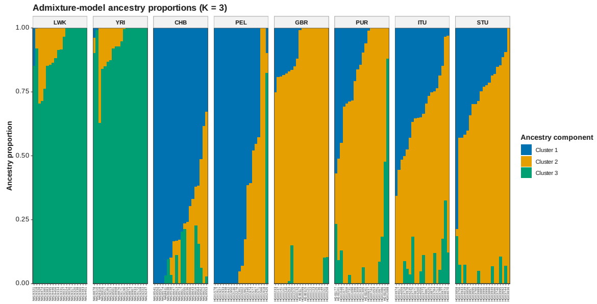
Figure 46: ADMIXTURE Q K 3
