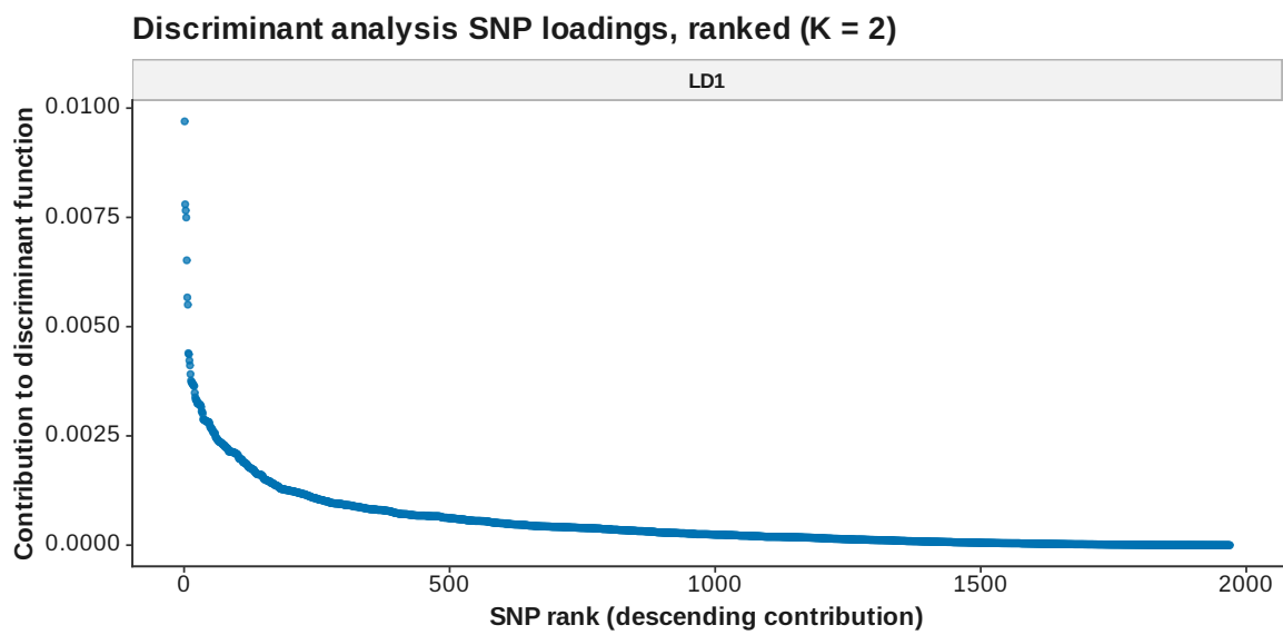
Figure 112: DAPC loadings ranked K 2
