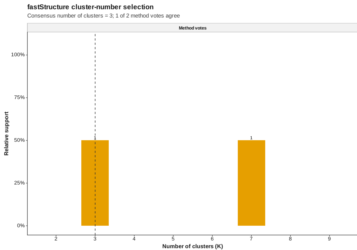
Figure 36: FastStructure cluster number selection
