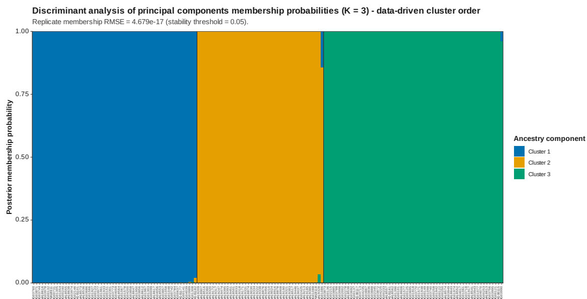
Figure 54: DAPC membership data driven K 3
