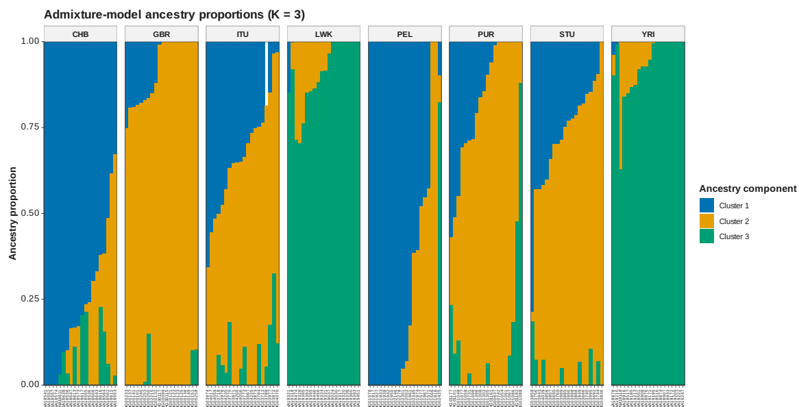
Figure 34: ADMIXTURE Q K 3
