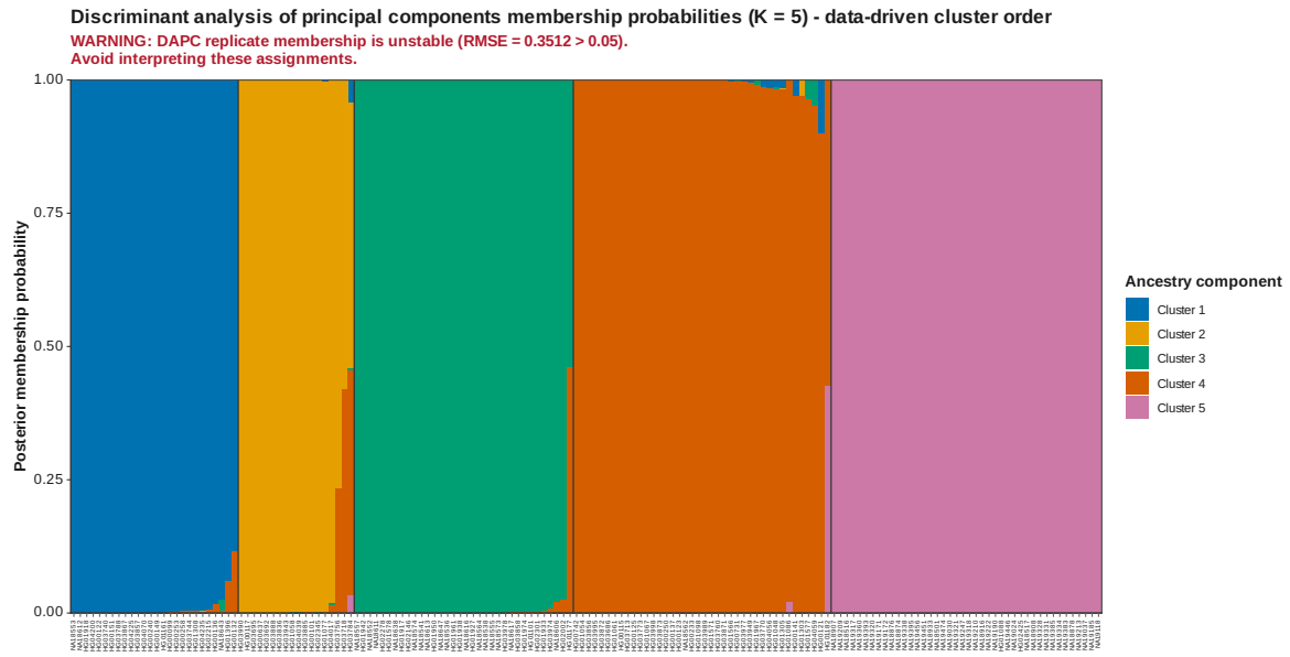
Figure 44: DAPC membership data driven K 5
