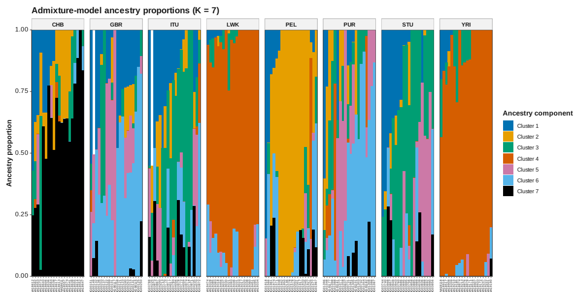
Figure 38: ADMIXTURE Q K 7
