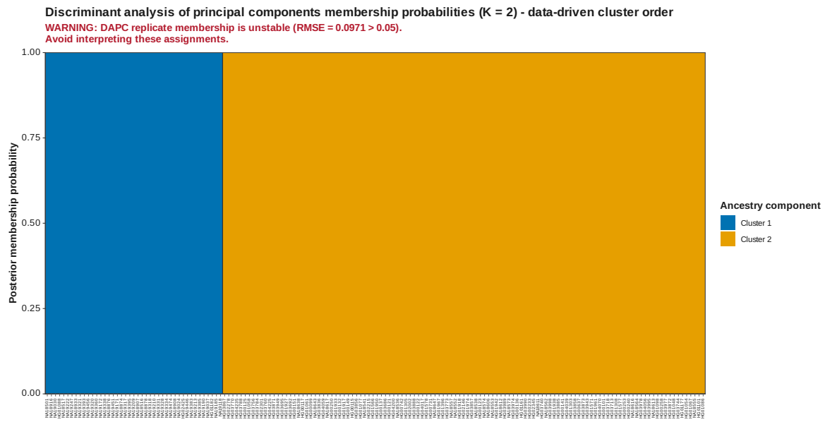
Figure 41: DAPC membership data driven K 2
