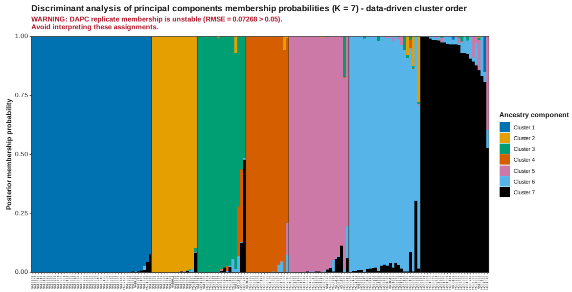
Figure 46: DAPC membership data driven K 7
