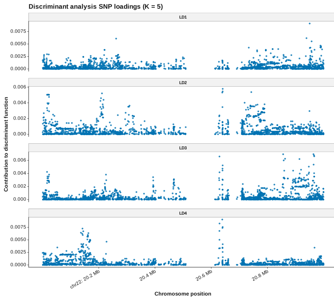
Figure 62: DAPC loadings manhattan K 5
