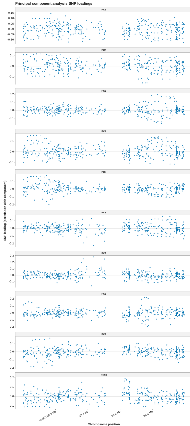
Figure 77: PCA loadings manhattan
