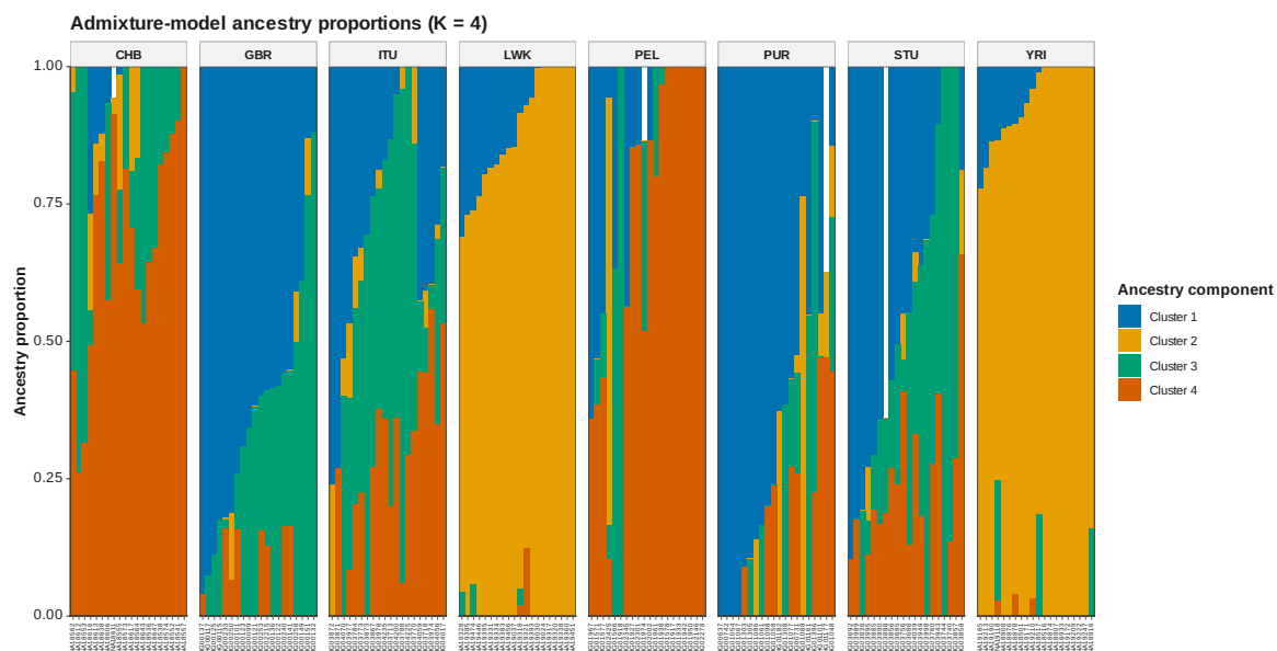
Figure 35: ADMIXTURE Q K 4
