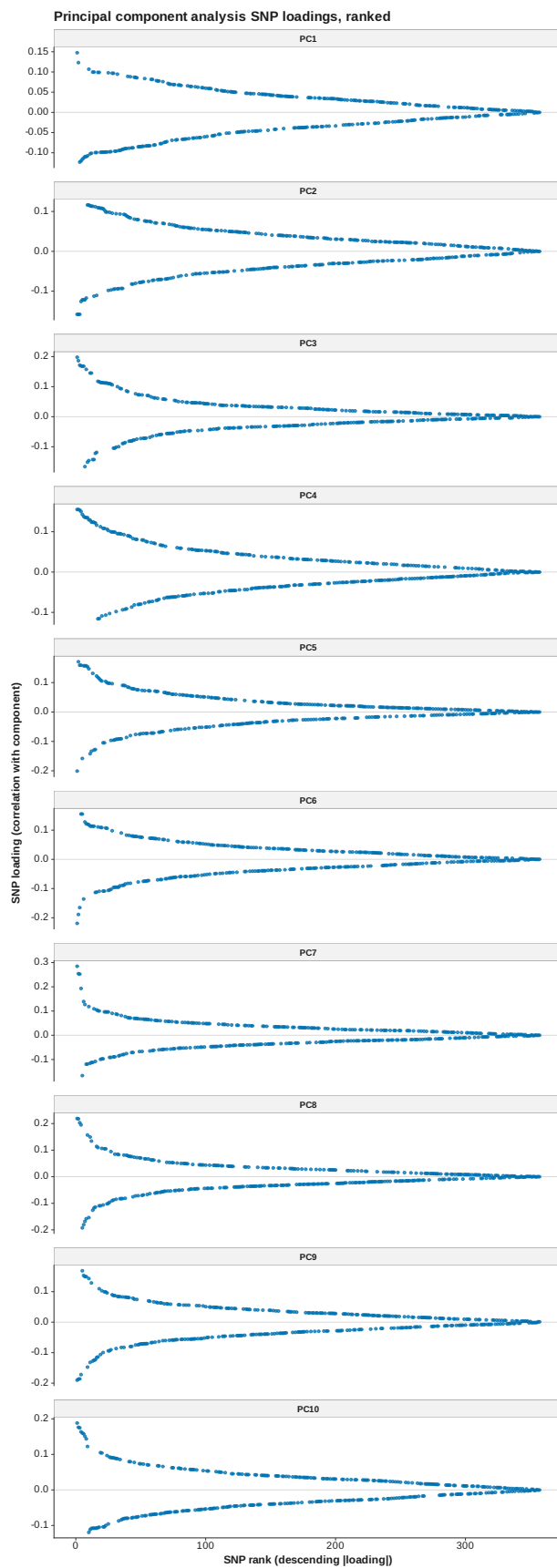
Figure 78: PCA loadings ranked
