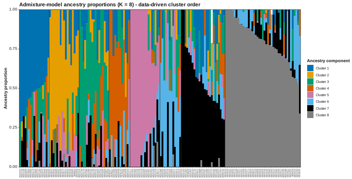
Figure 31: ADMIXTURE Q data driven K 8
