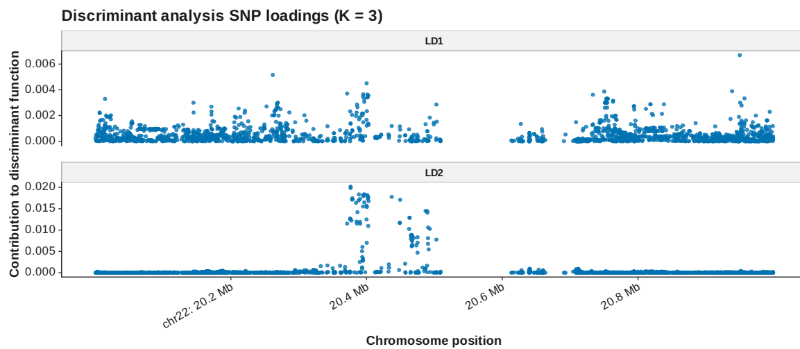
Figure 60: DAPC loadings manhattan K 3
