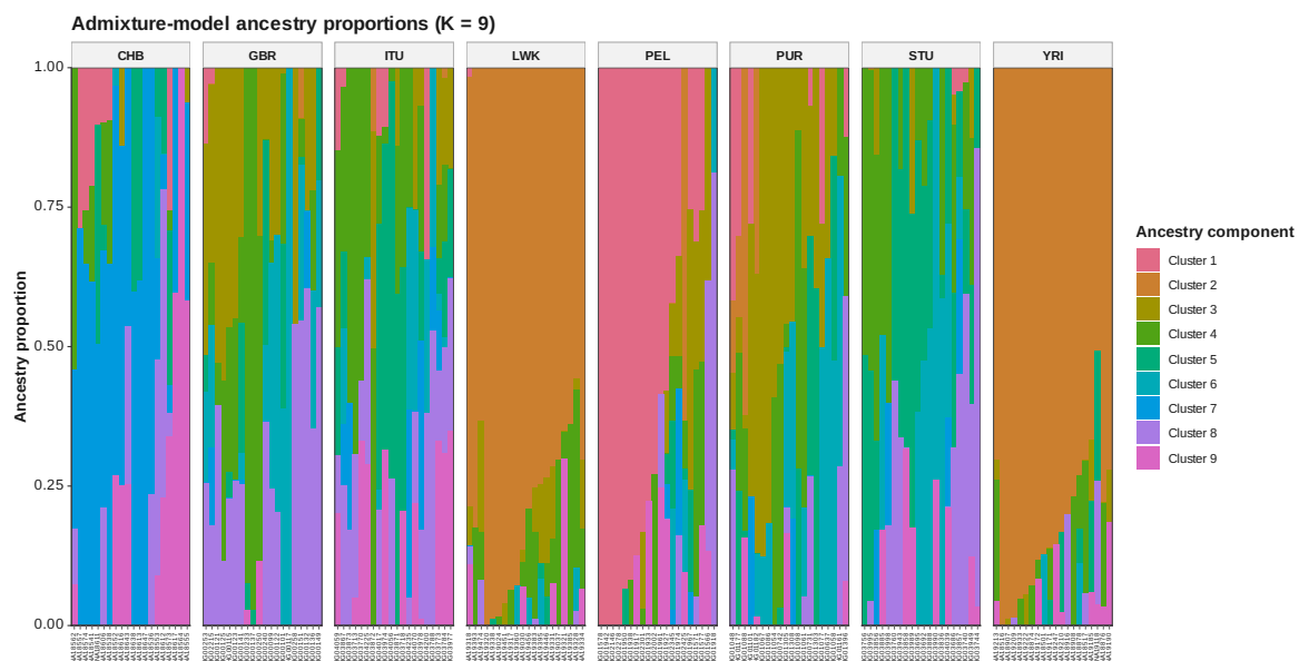
Figure 40: ADMIXTURE Q K 9
