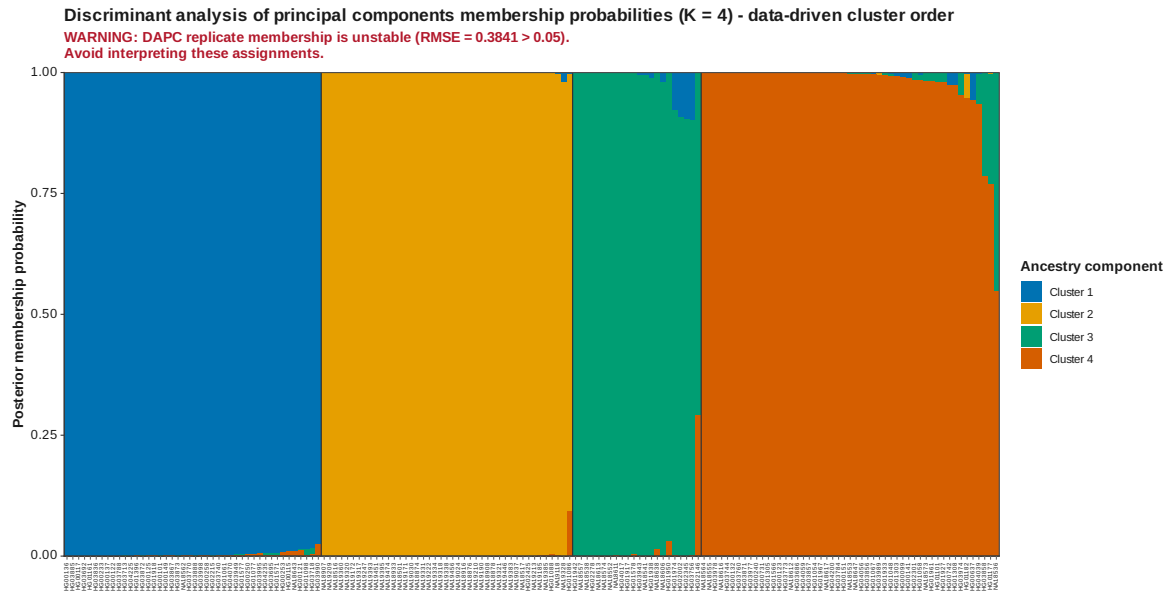
Figure 43: DAPC membership data driven K 4
