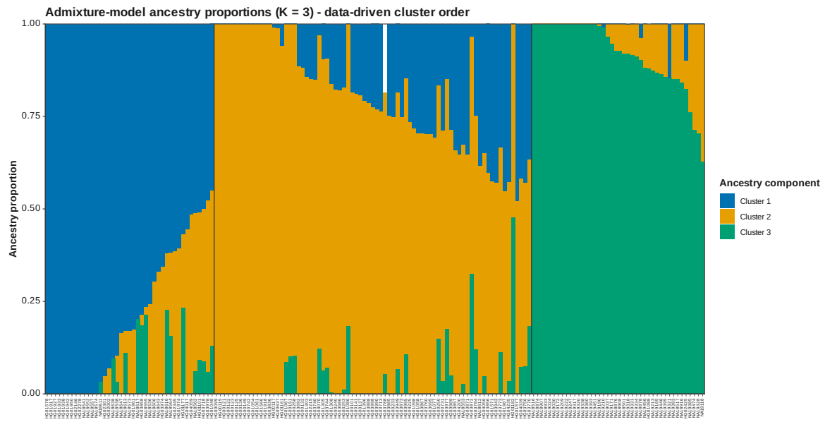
Figure 26: ADMIXTURE Q data driven K 3
