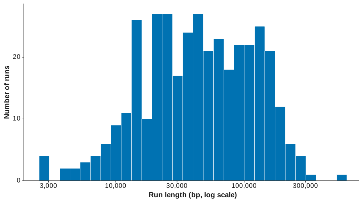
Figure 117: ROH length distribution
