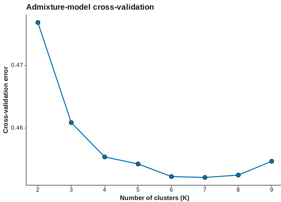
Figure 24: ADMIXTURE CV
