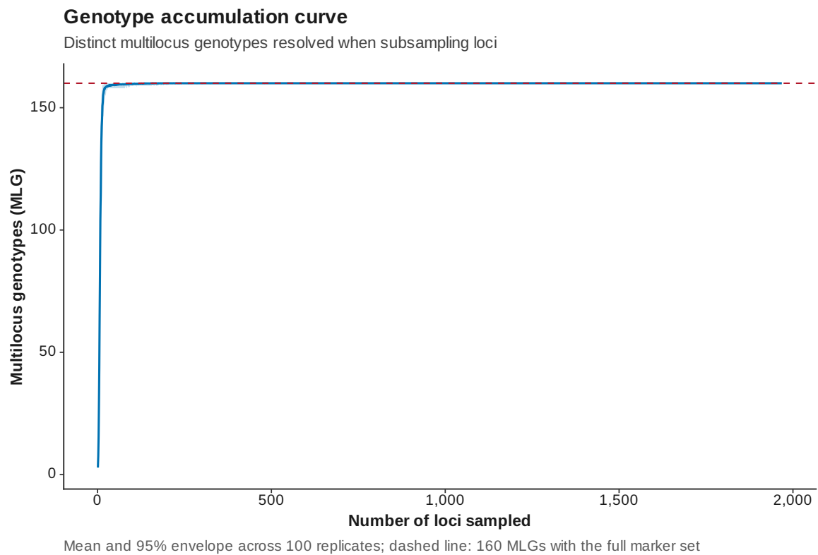
Figure 133: Genotype accumulation curve
