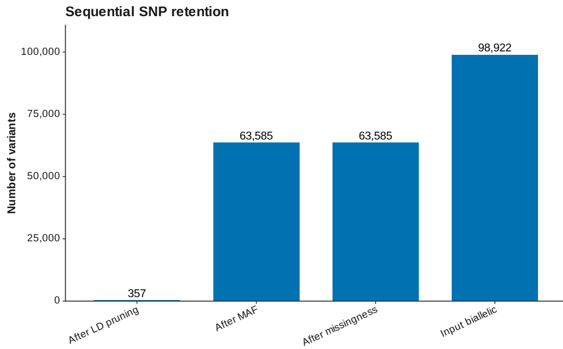
Figure 4: SNP retention
