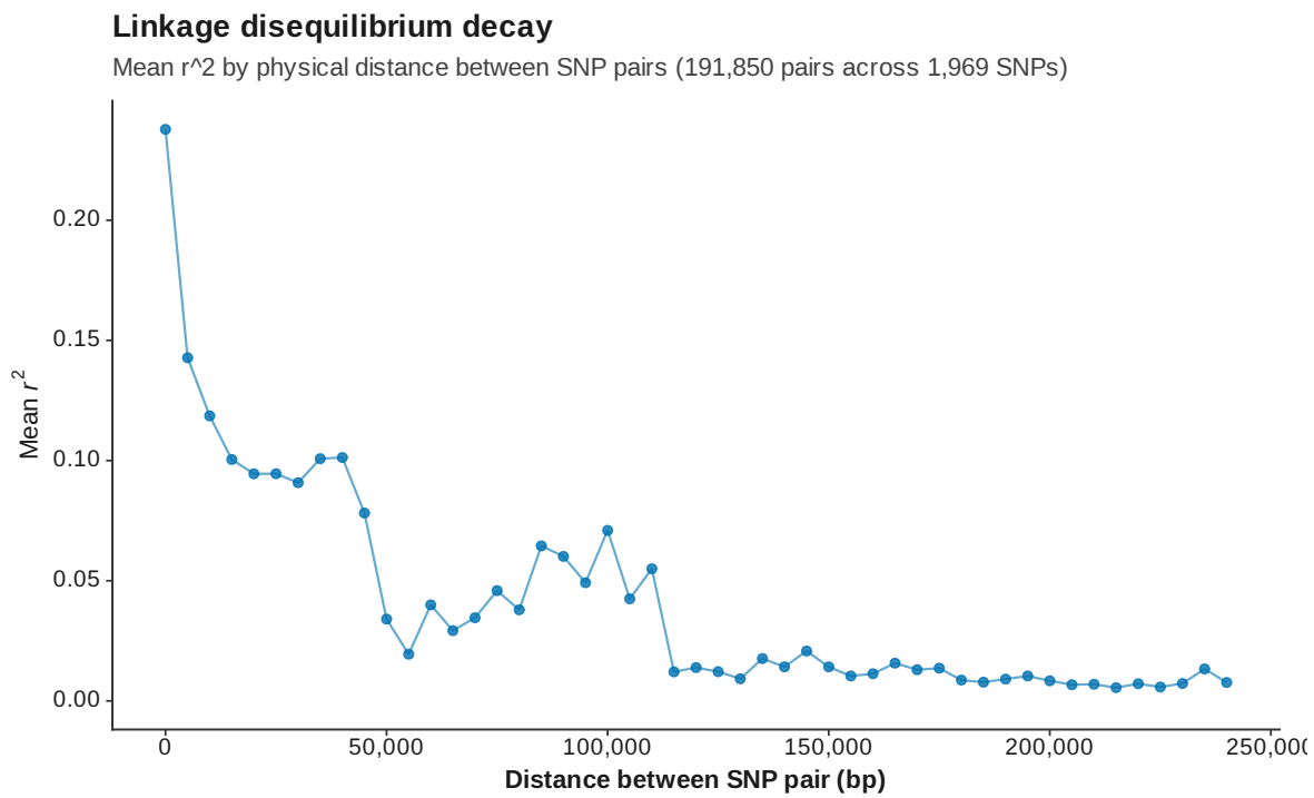
Figure 122: LD decay
