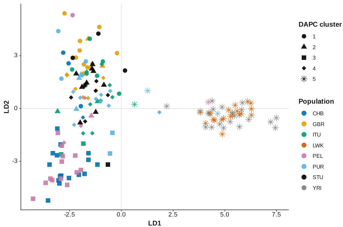
Figure 16: DAPC K 5
