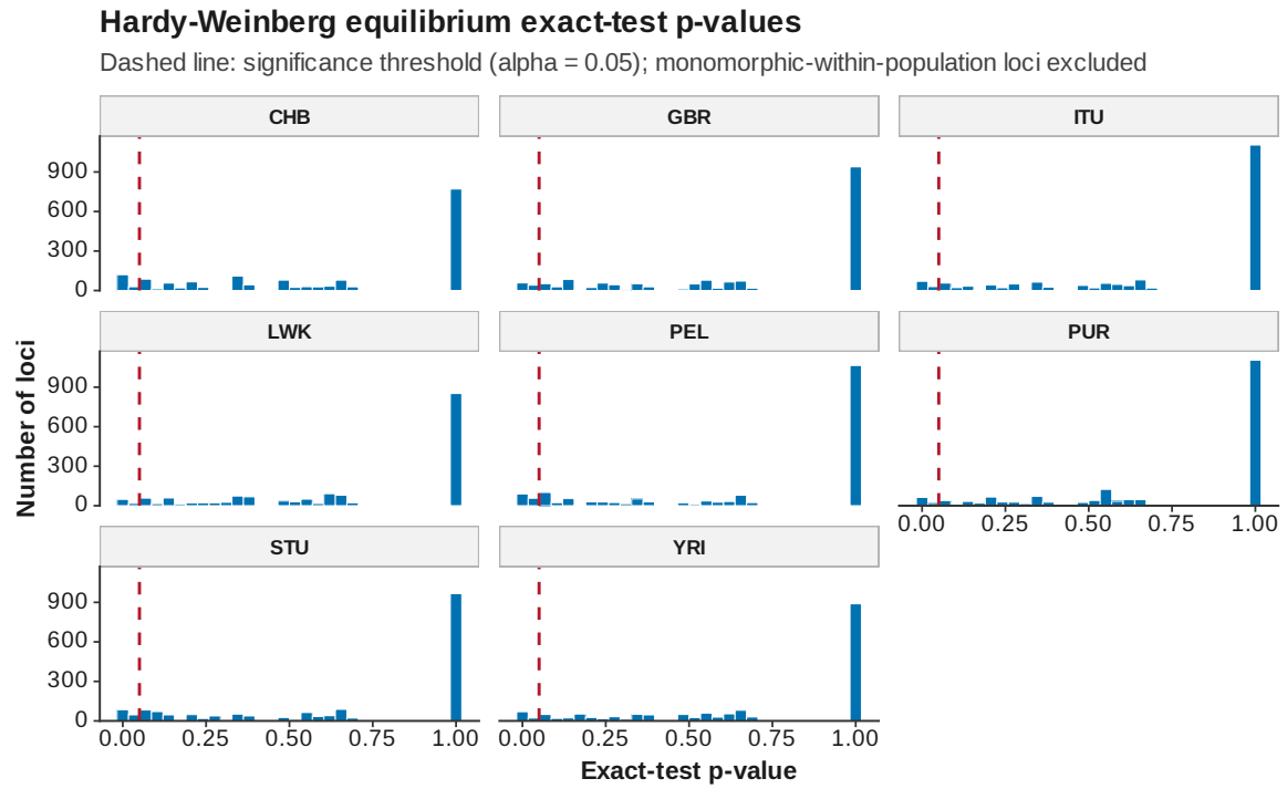
Figure 114: HWE pvalues
