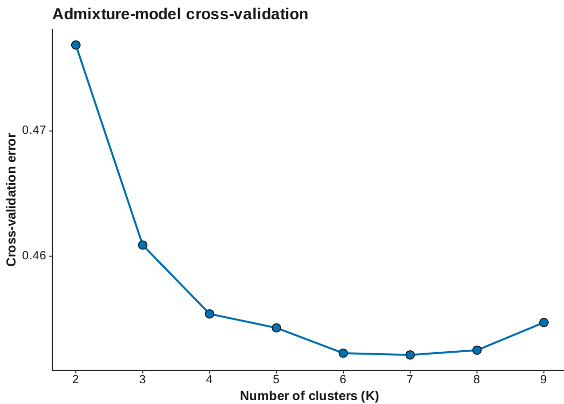
Figure 23: ADMIXTURE CV
