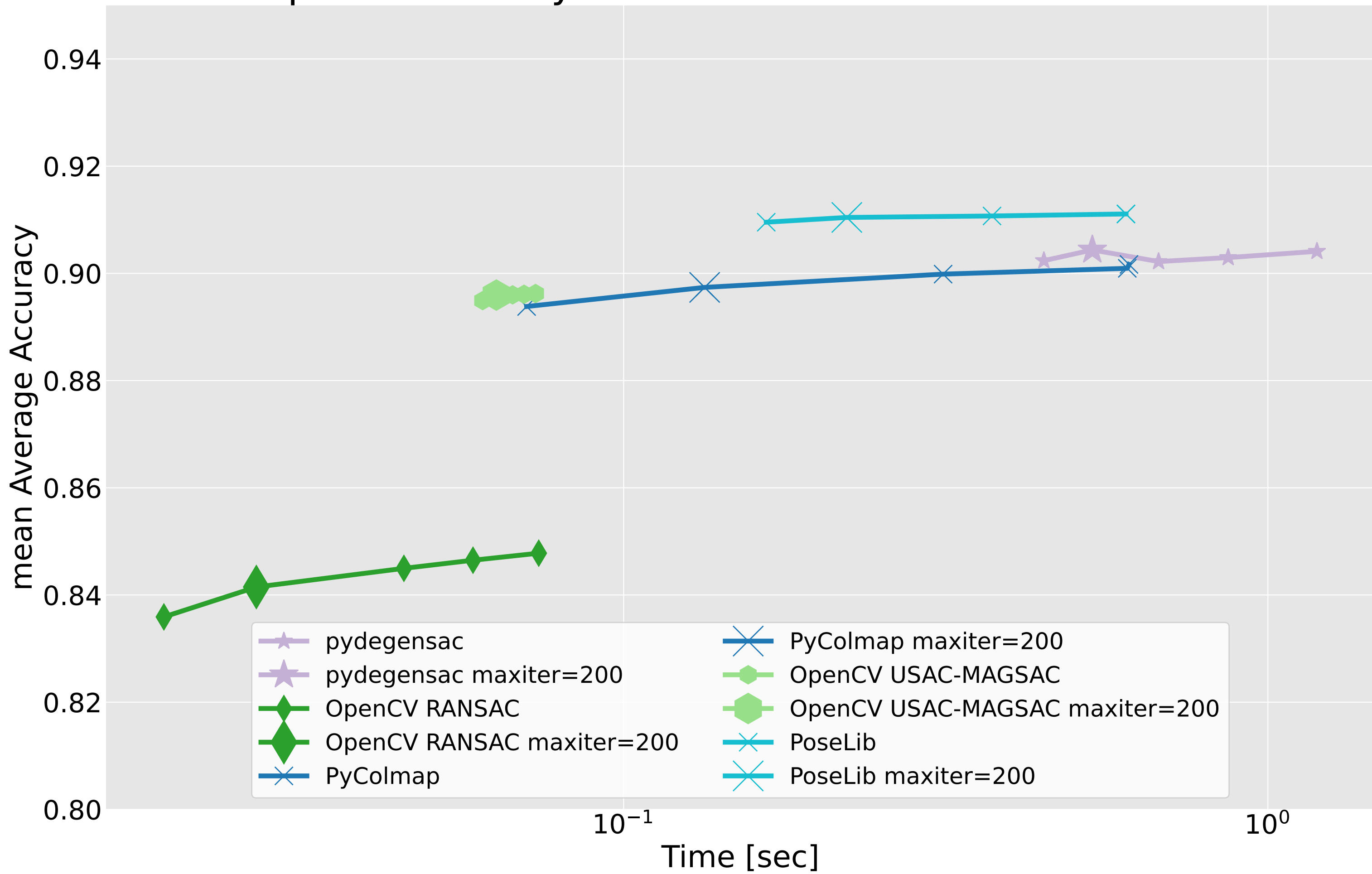
Speed-Accuracy Tradeoff with 20k RoMa matches
