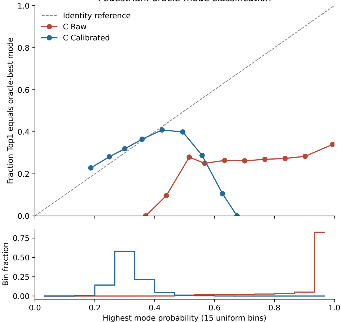
Pedestrian: oracle-mode classification
