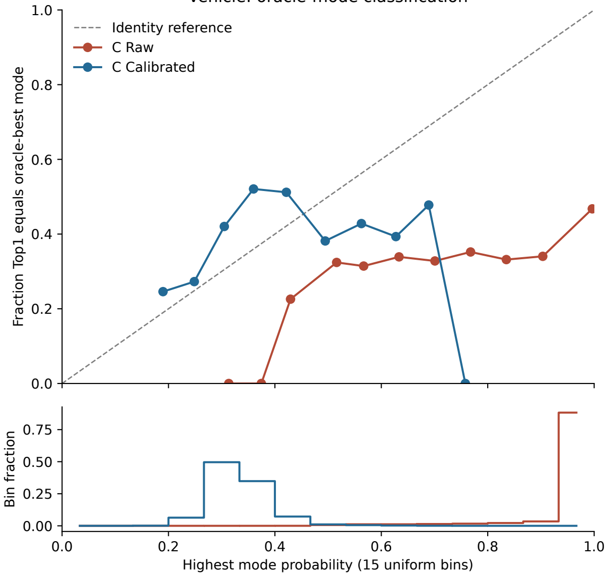
Vehicle: oracle-mode classification
