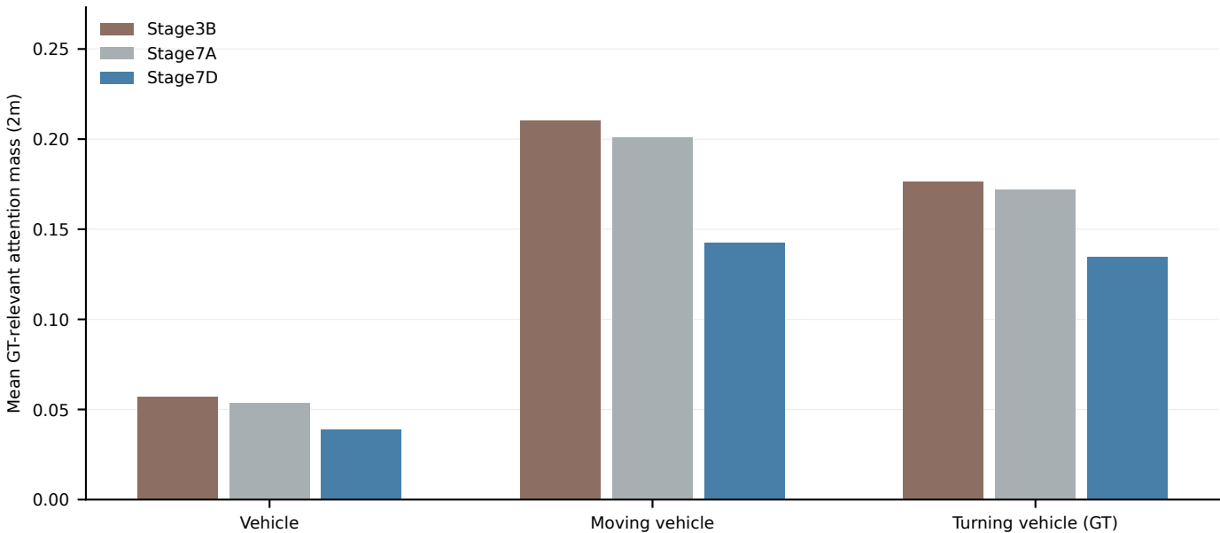
GT-relative lane attention: actor-pooled full-horizon VAL
