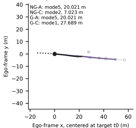
f MovingVehicle high-cost failure Fold3 | \Delta(G-C - NG-C) = +20.6655 m
