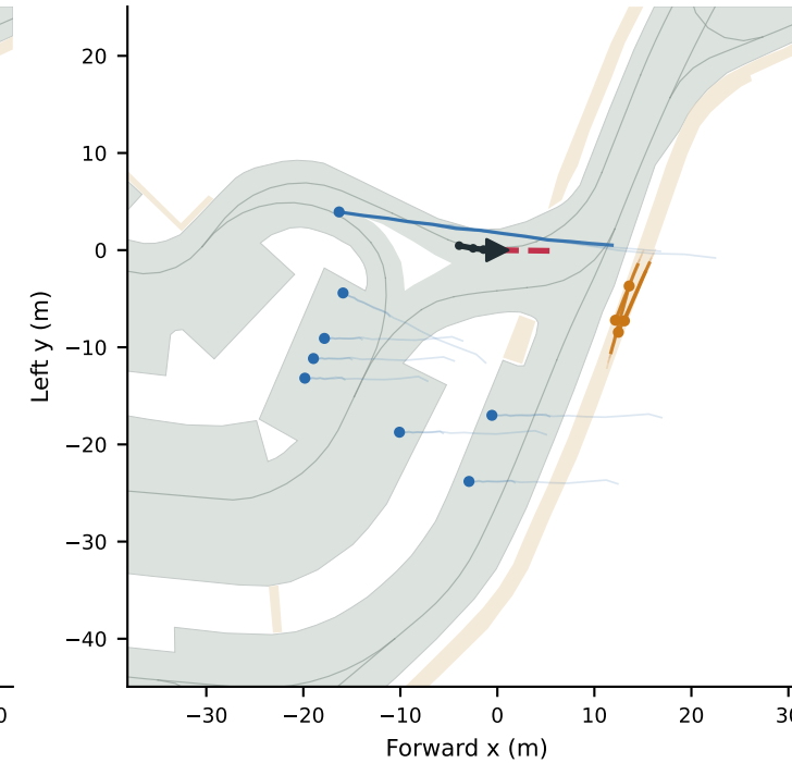
4. Static map + forecasts CV ego from observed history
