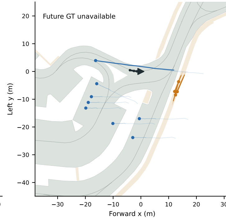
3. Static map + forecasts Recorded ego future = EvaluationOnly
