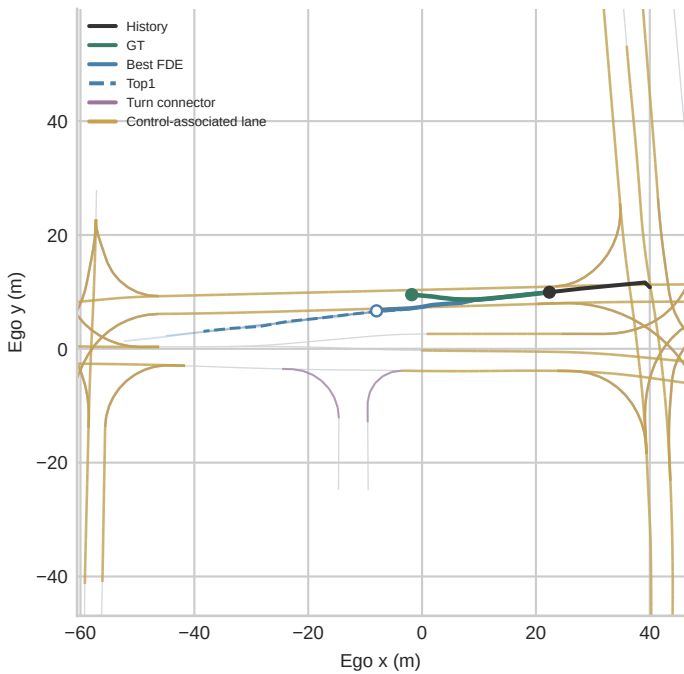
Stage3B minFDE6=6.81m
