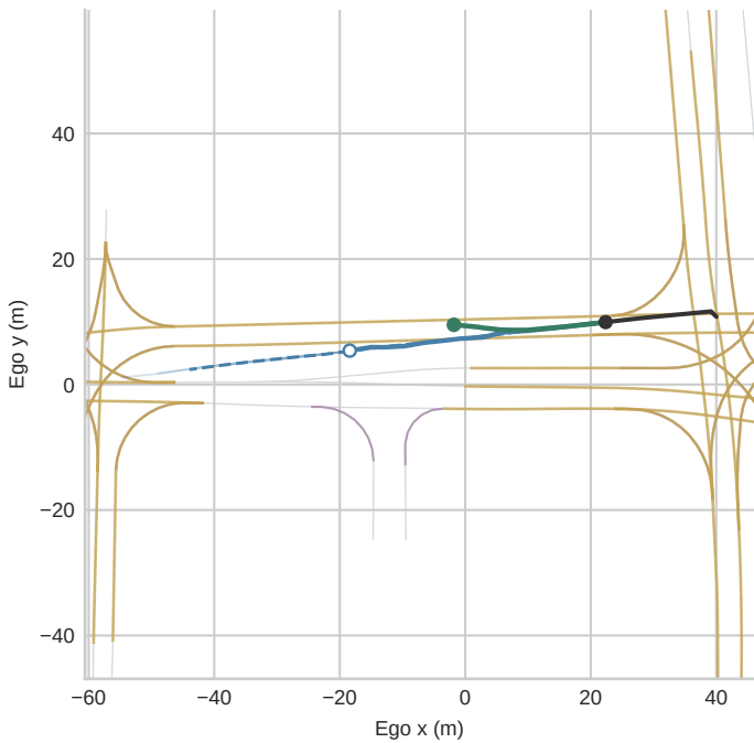
Stage7A minFDE6=17.10m
