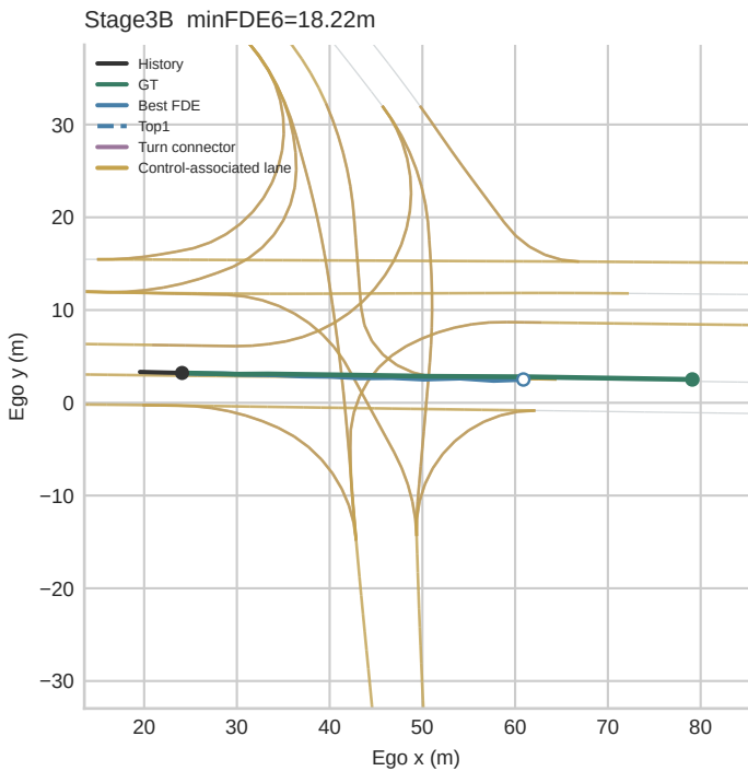
Traffic-control context: improvement, \Delta=-6.64\text{m} scene-0097; same actor, frozen map and axes
