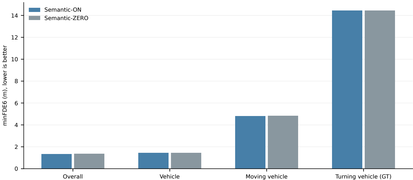
Same Stage7A checkpoint: semantic input inference ablation
