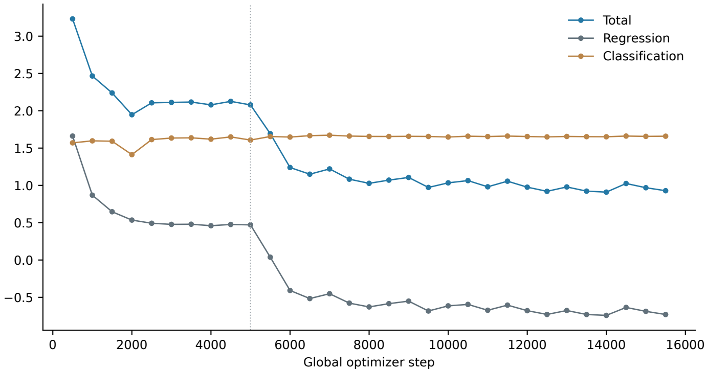
Mean batch loss over preceding 500 updates
