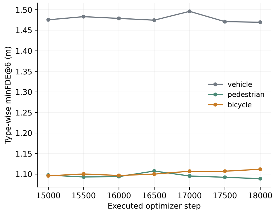
b Per-type validation
