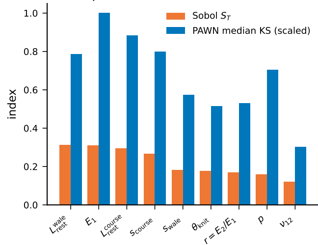
(c) cable \Delta H : variance-based vs moment-independent Spearman rank correlation 0.78
