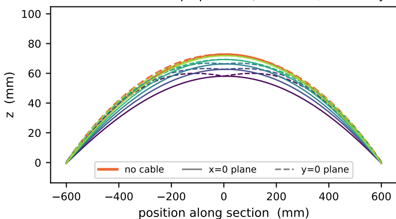
Stitch structure I — shape profiles (solid= x=0 , dashed= y=0 )
