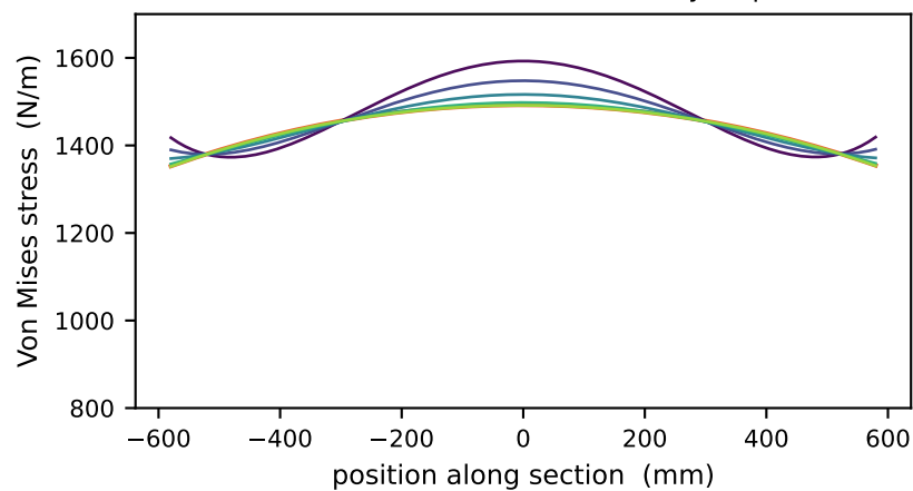
Stitch structure I — section stress ( y=0 plane)
