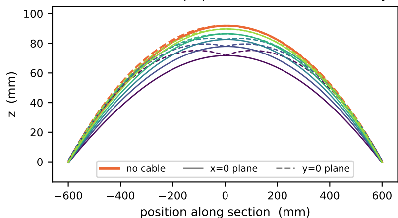
Stitch structure II — shape profiles (solid= x=0 , dashed= y=0 )
