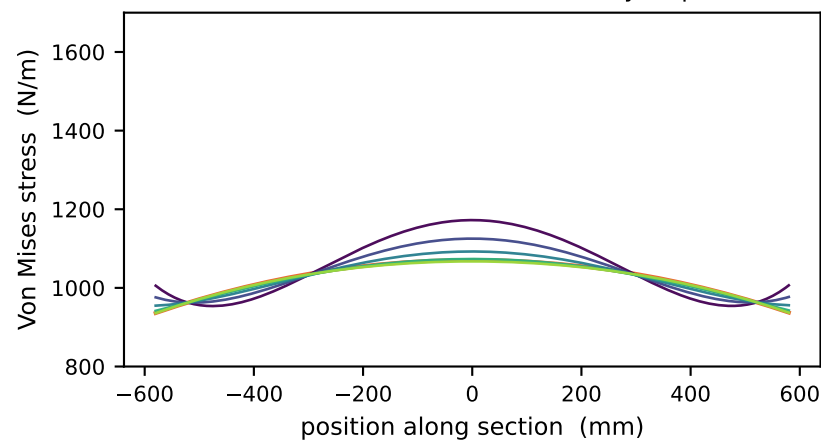
Stitch structure II — section stress ( y=0 plane)
