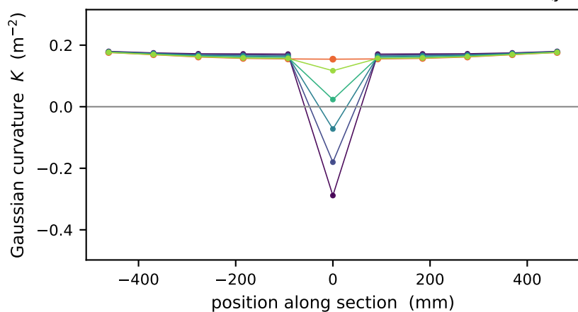
Stitch structure I — Gaussian curvature across the cable ( y=0 )
