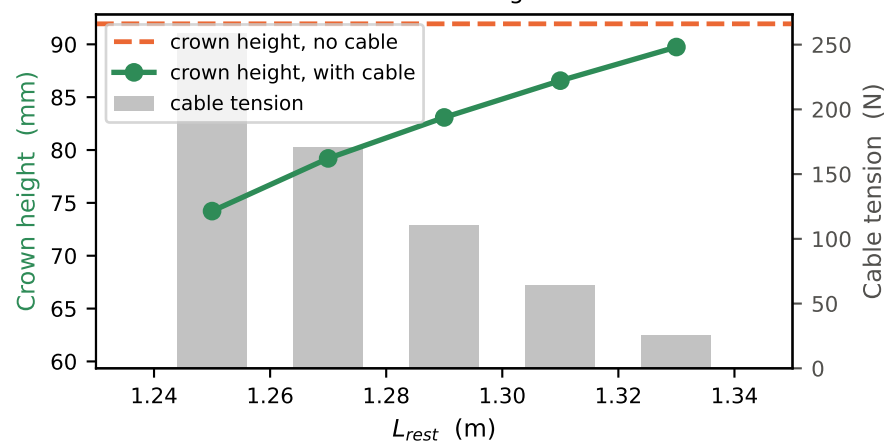
Stitch structure II — crown height &amp; cable tension
