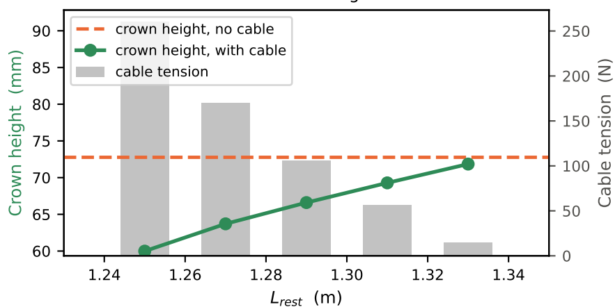
Stitch structure I — crown height &amp; cable tension
