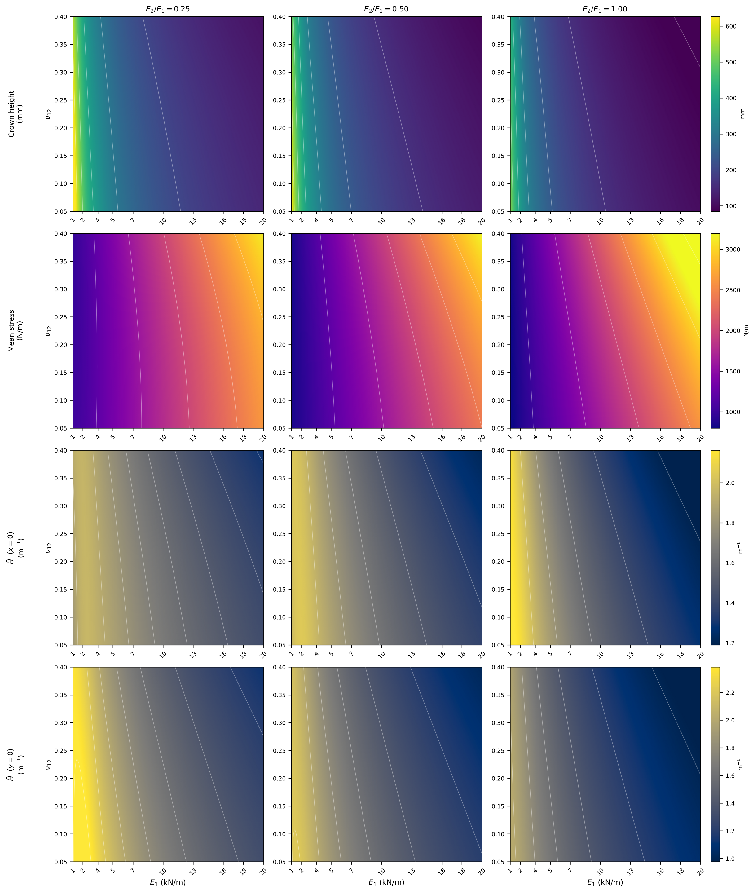
Fig S — E_1 \times \nu_{12} response surfaces (3 anisotropy slices) s_f = 1.1 , p = 1000 Pa, \theta_{\text{knit}} = 0^\circ
