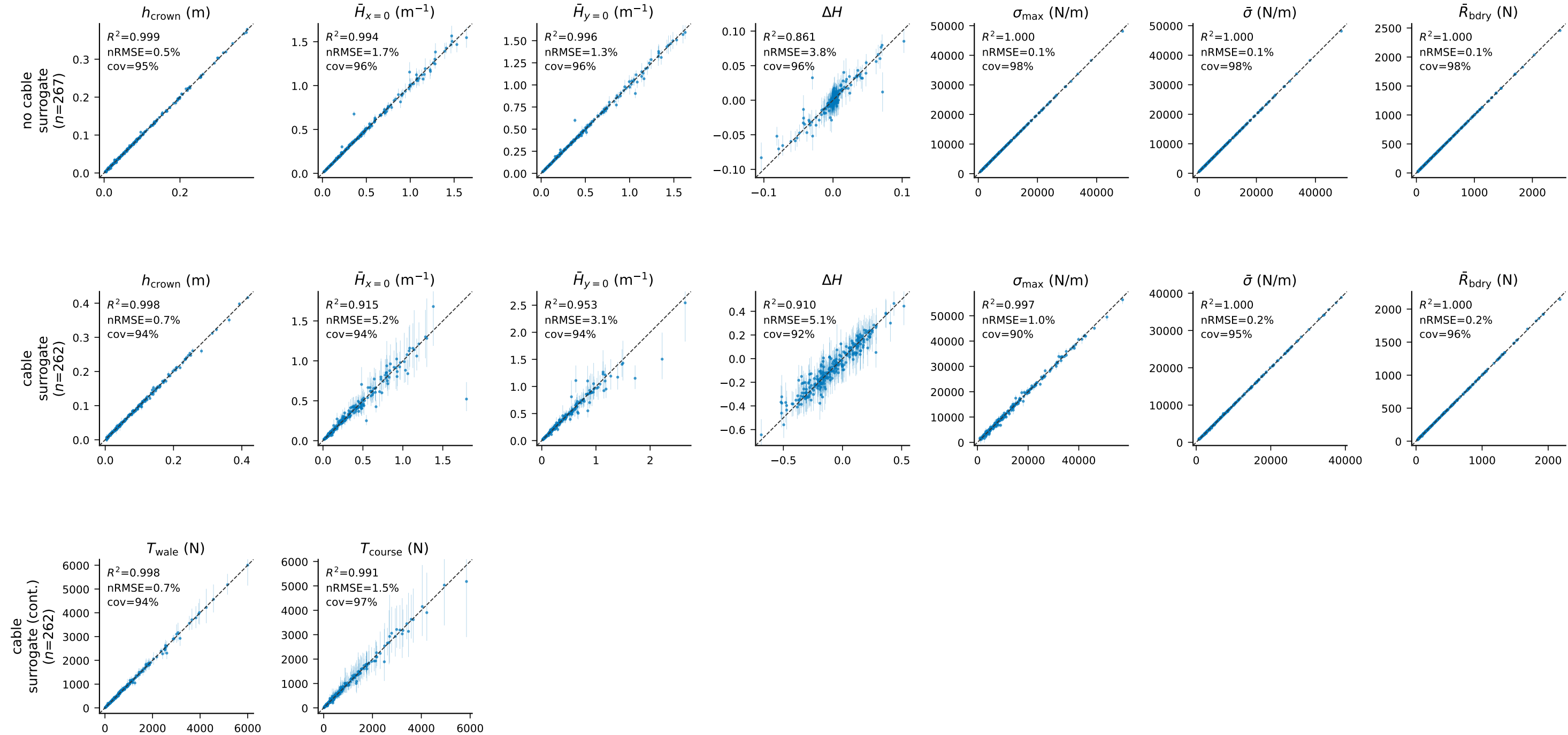
Surrogate accuracy on held-out runs: prediction vs FEA, with 95% predictive intervals (validity box, s \geq 0.95 )
