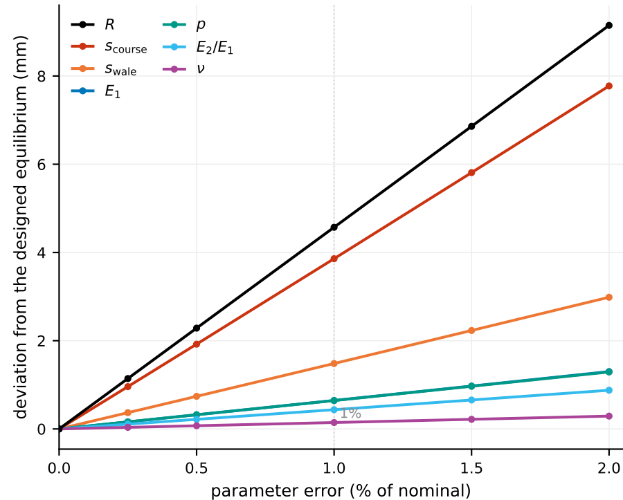
(a) circular dome
