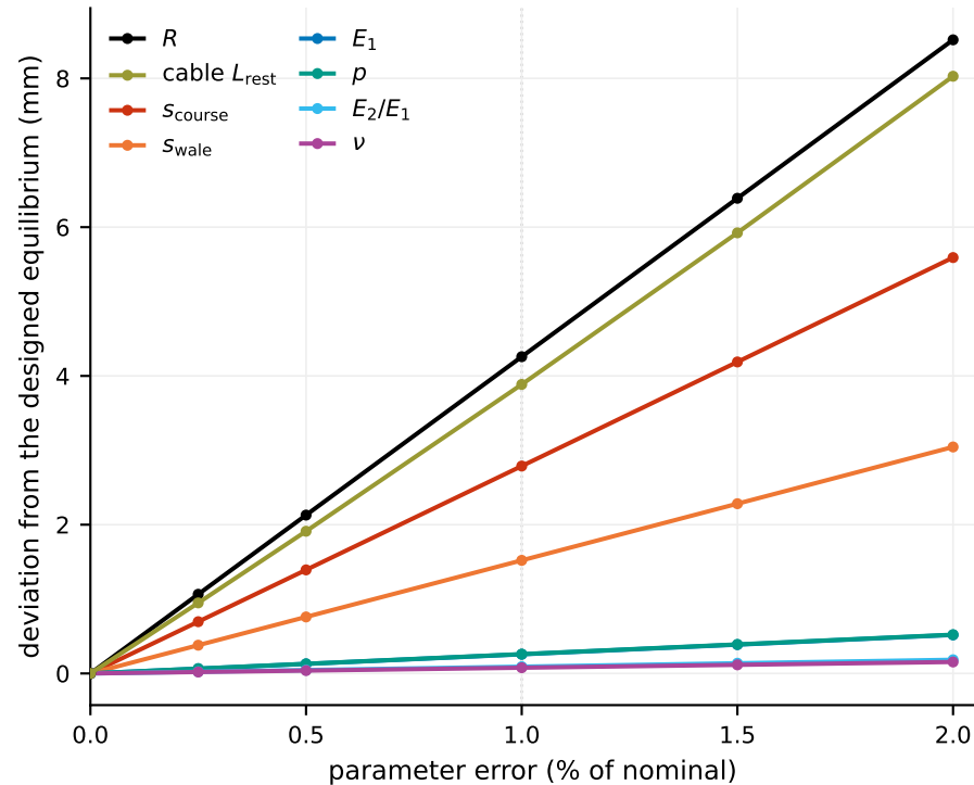
(b) creased shell as designed: optimised factors + crease cable
