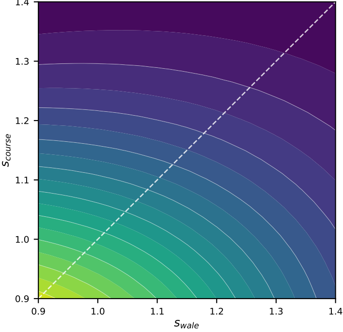
Motif 1 ( E_2/E_1 = 2.50 ) — Section stress x = 0
