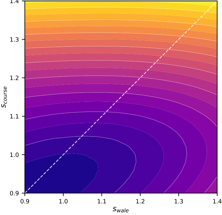
Motif 1 ( E_2/E_1 = 2.50 ) — Section stress y = 0
