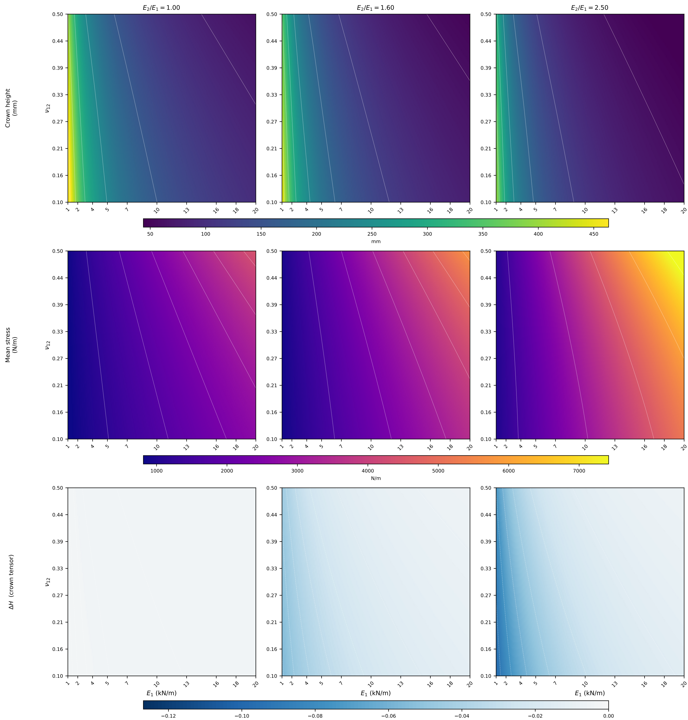
Fig S — E_1 \times v_{12} response surfaces, s_f = 1.1 , p = 1000 Pa, \theta_{\text{knit}} = 0^\circ
