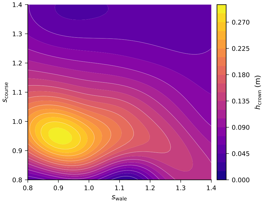
Response surface — h_{\text{crown}} (m), Motif 1 (at median \theta_{\text{knit}} , p )
