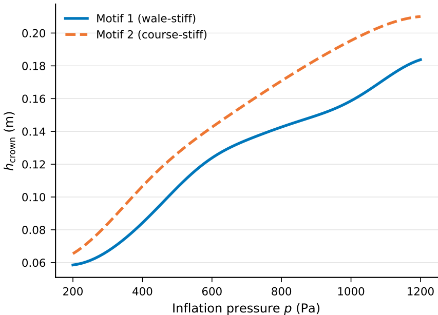
h_{\text{crown}} vs. inflation pressure
