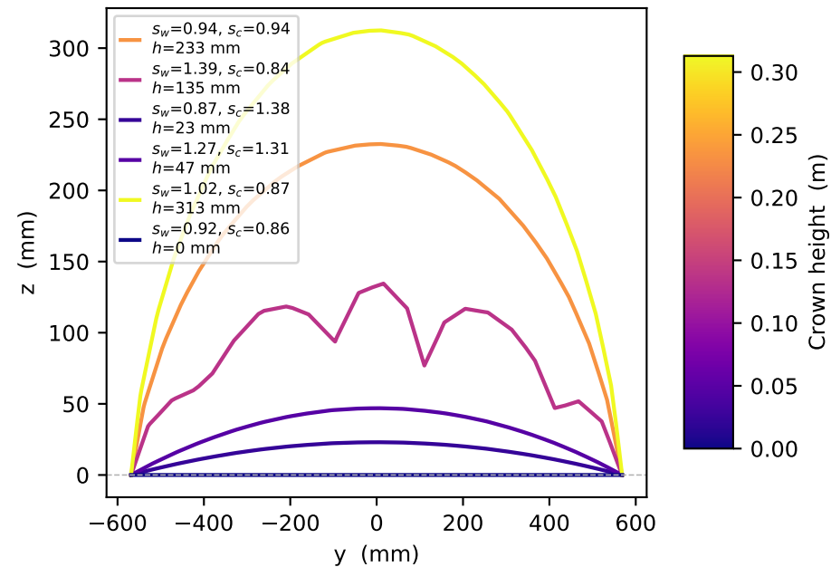
YZ cross-sections — motif1 cable
